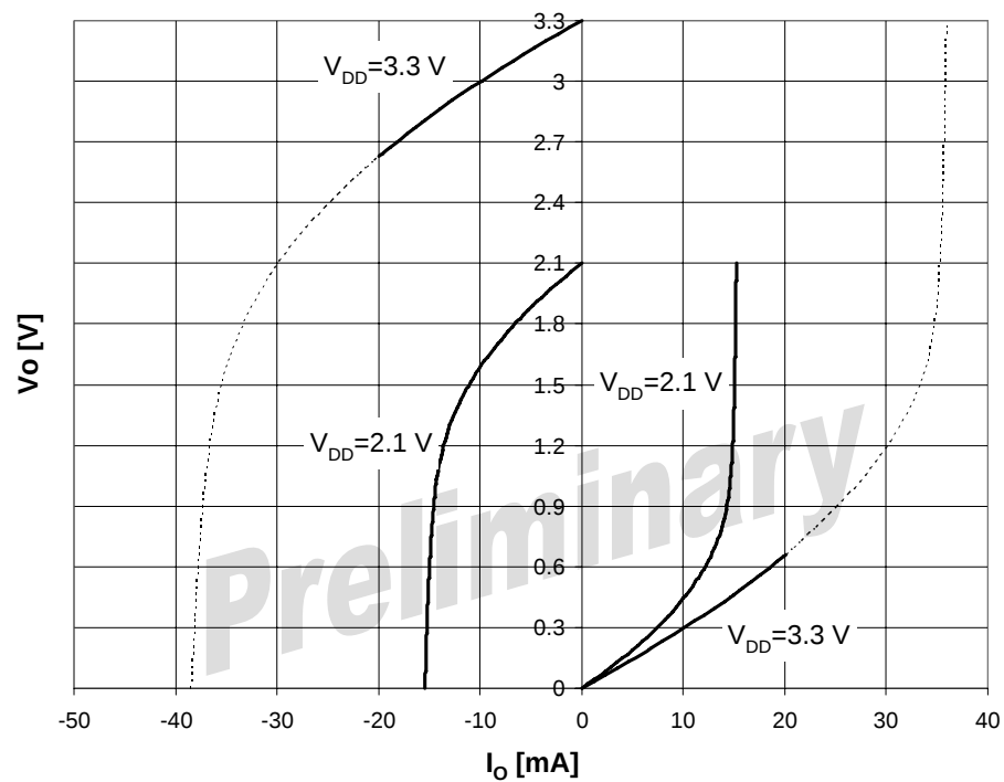
Figure 23: Typical output characteristic ( T_j = 25^\circ\text{C} )
