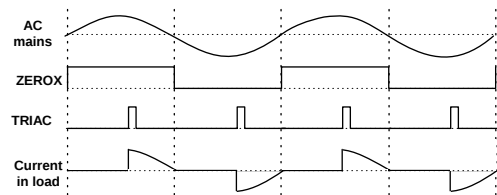
Figure 12: Typical triac waveforms
