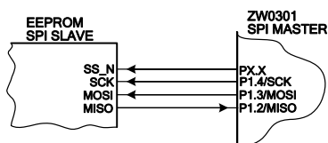
Figure 20: Typical interface to EEPROM
