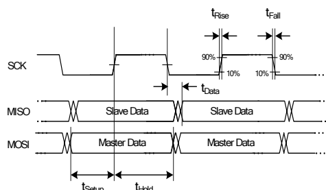
Figure 25: SPI timing
