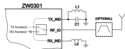
Figure 7: RF interface in typical application
