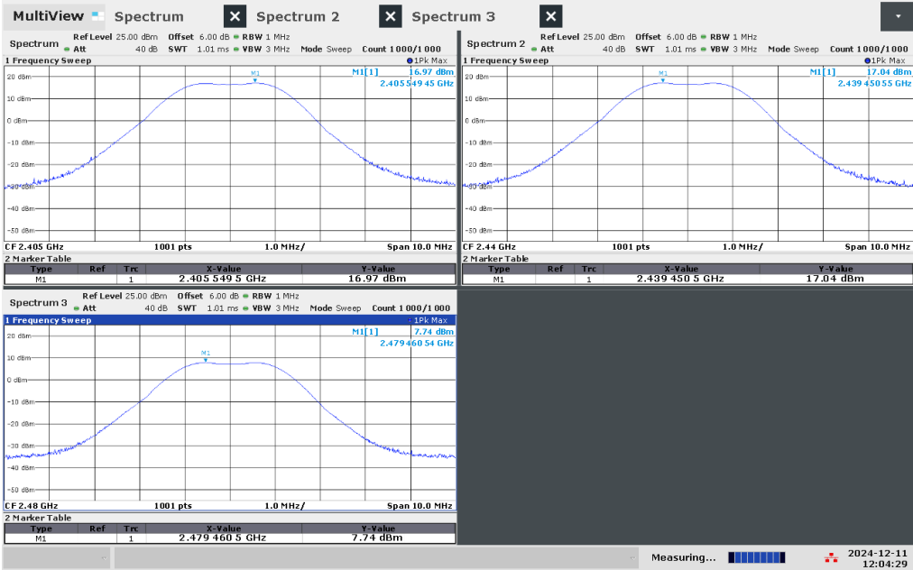
Figure 4.2.3 (iii) Conducted RF Power Plots
