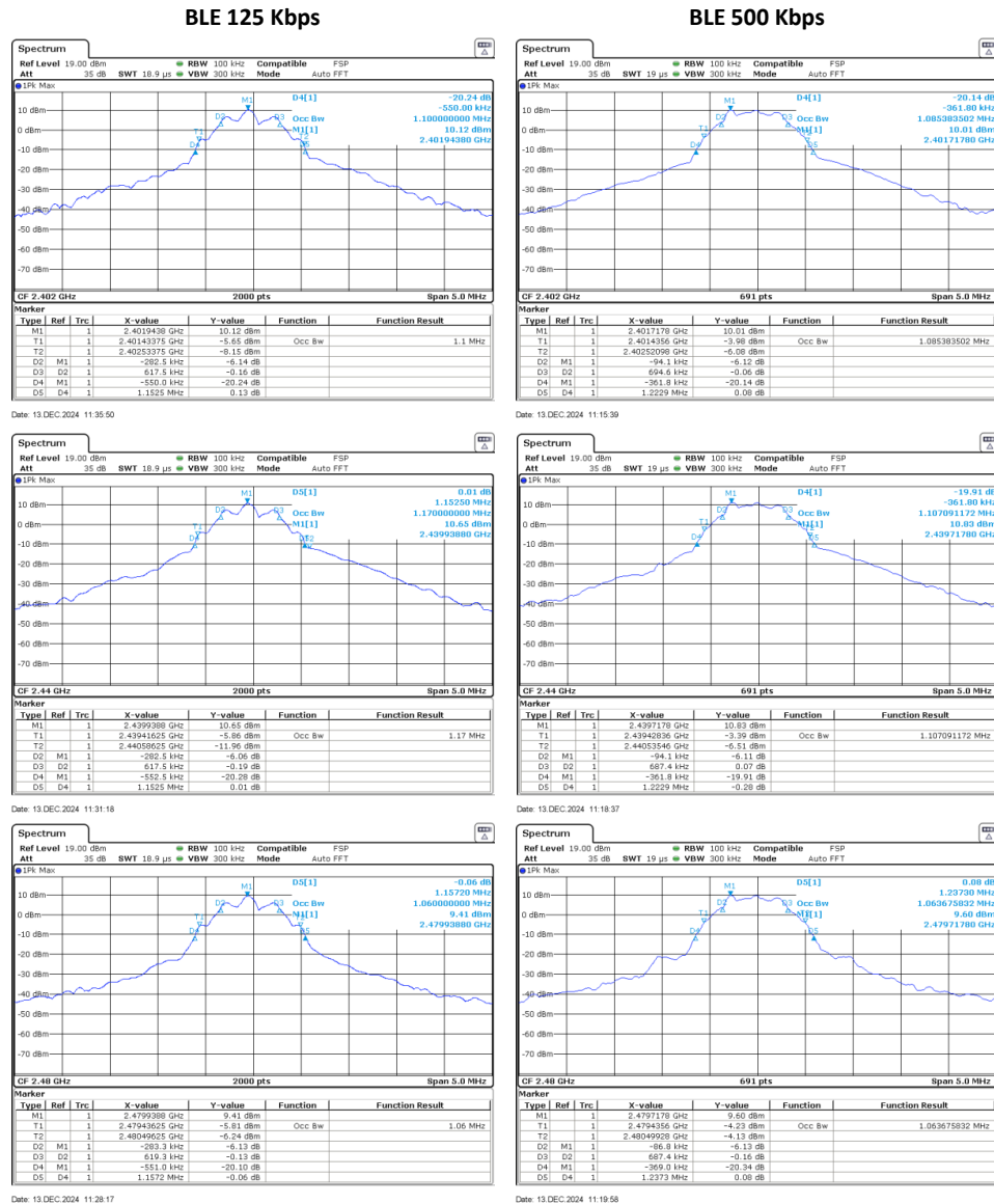
Figure 4.2.2 (i) Example Intentional Emission Bandwidth Plots.
