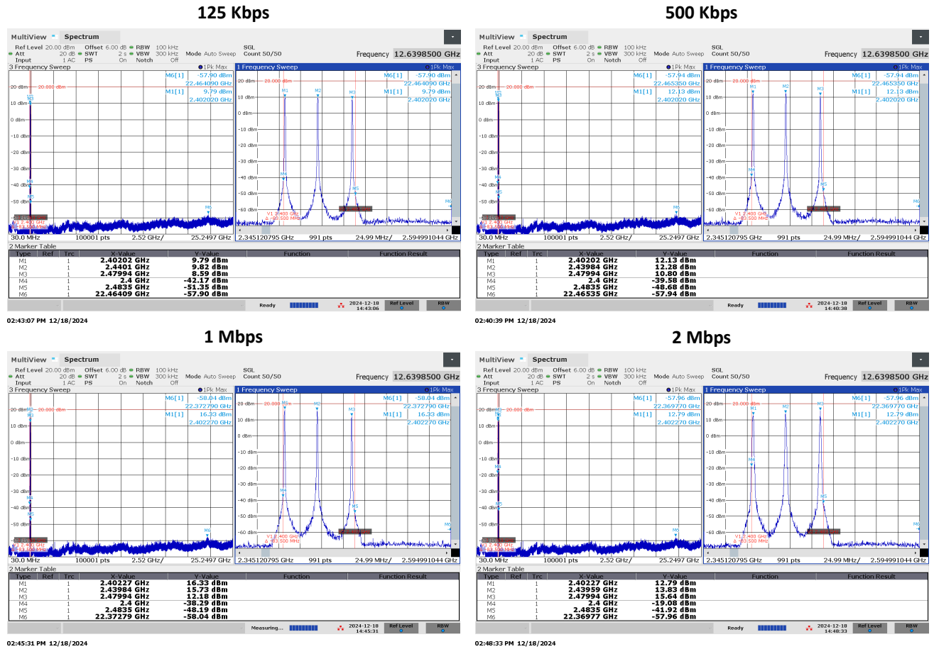
Figure 4.3.2 (i) Worst Case Transmitter OOB Emissions Measured.
