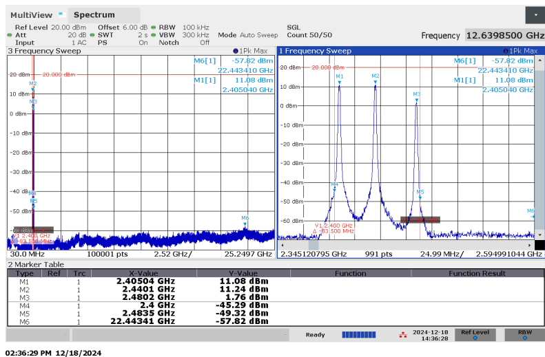
Figure 4.3.2 (ii) Worst Case Transmitter OOB Emissions Measured.
