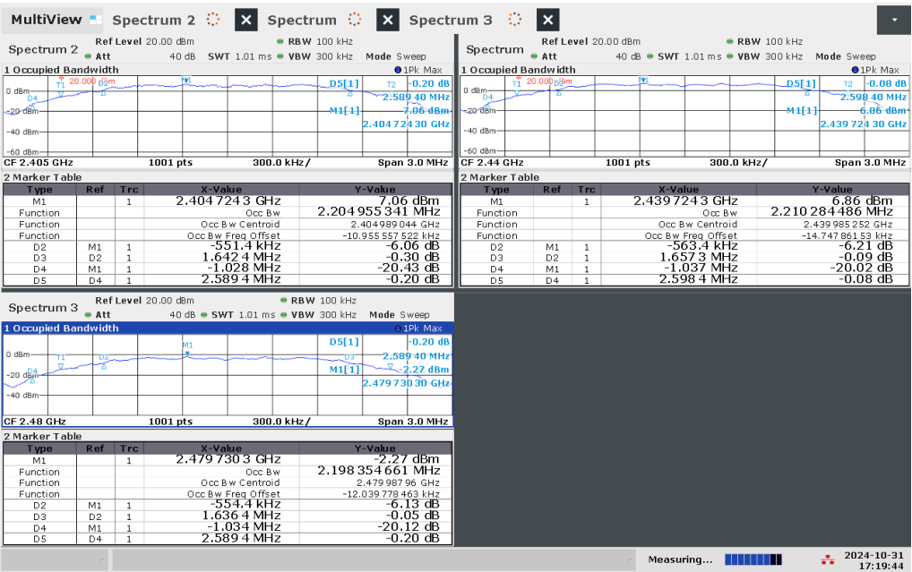
Figure 4.2.2 (iii) Example Intentional Emission Bandwidth Plots.
