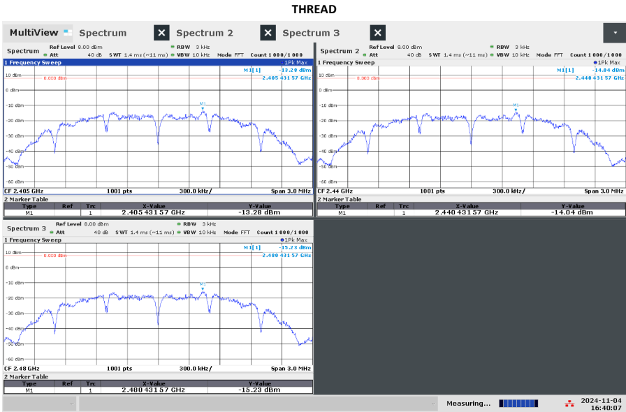
Figure 4.2.4 (iii) Power Spectral Density Plots.
