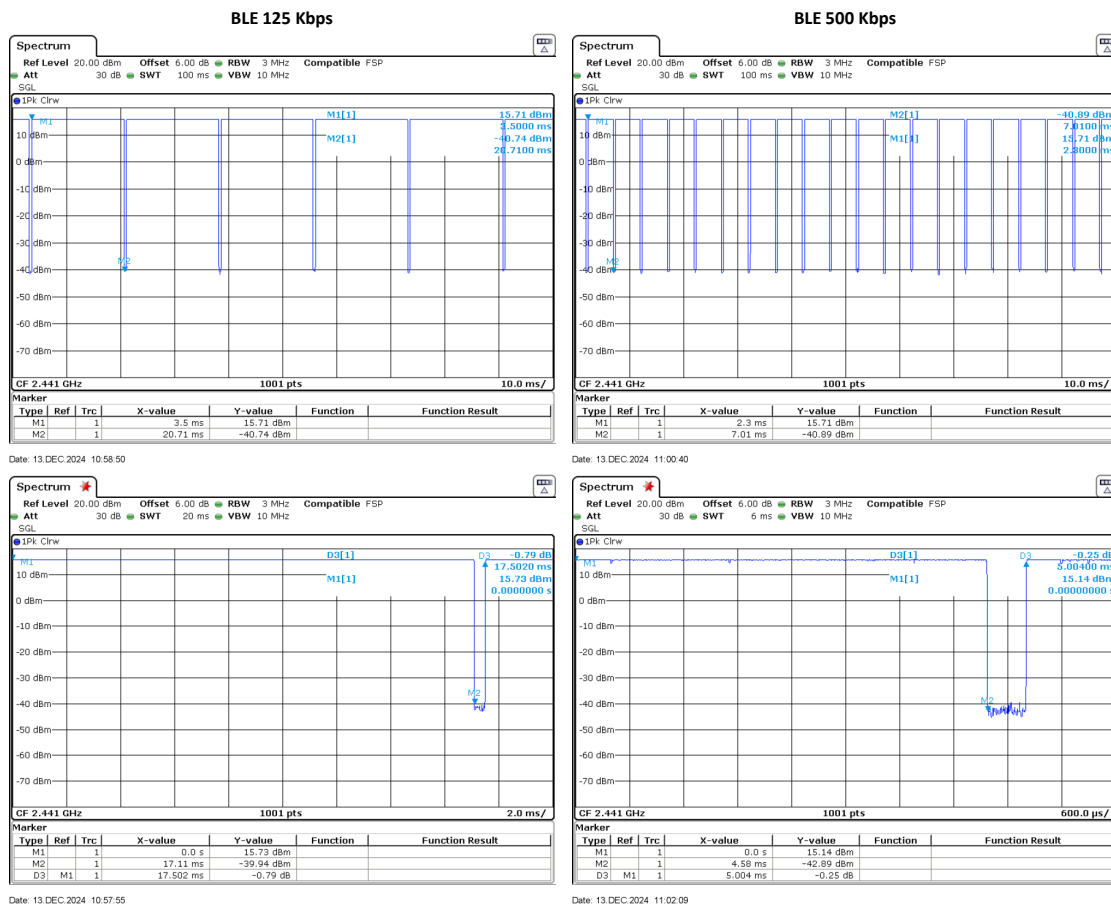
Figure 4.2.1 (i) Example Pulsed Emission Characteristics (Duty Cycle).
