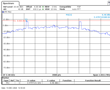
Figure 4.2.4 (i) Power Spectral Density Plots.
