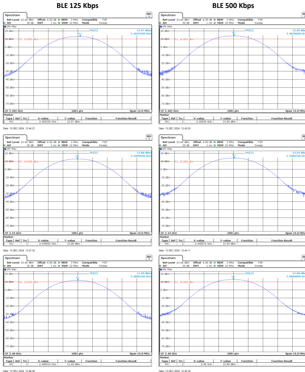
Figure 4.2.3 (i) Conducted RF Power Plots
