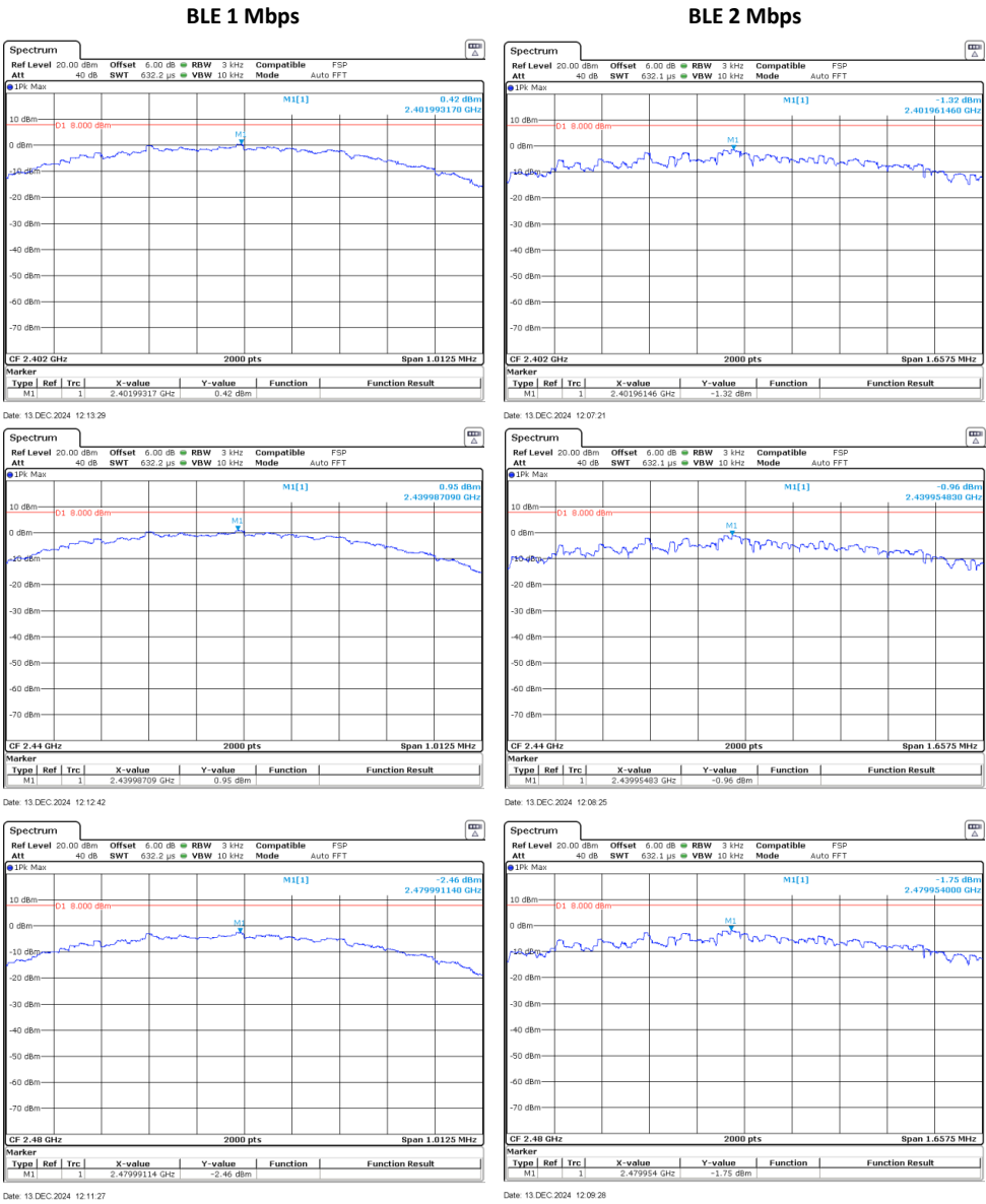
Figure 4.2.4 (ii) Power Spectral Density Plots.
