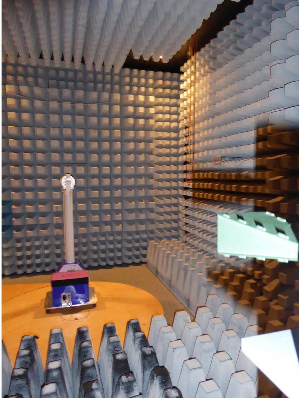
181323_SetRadE11.JPG: Test setup fully anechoic chamber; EVB-ANNA-B112E#143, 18 – 26.5 GHz
