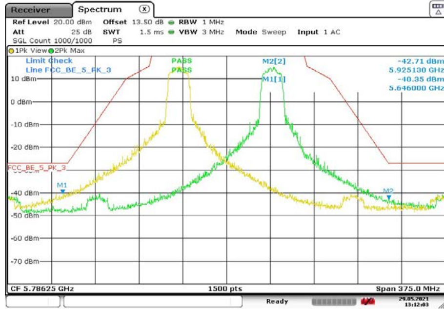
Antenna 0
