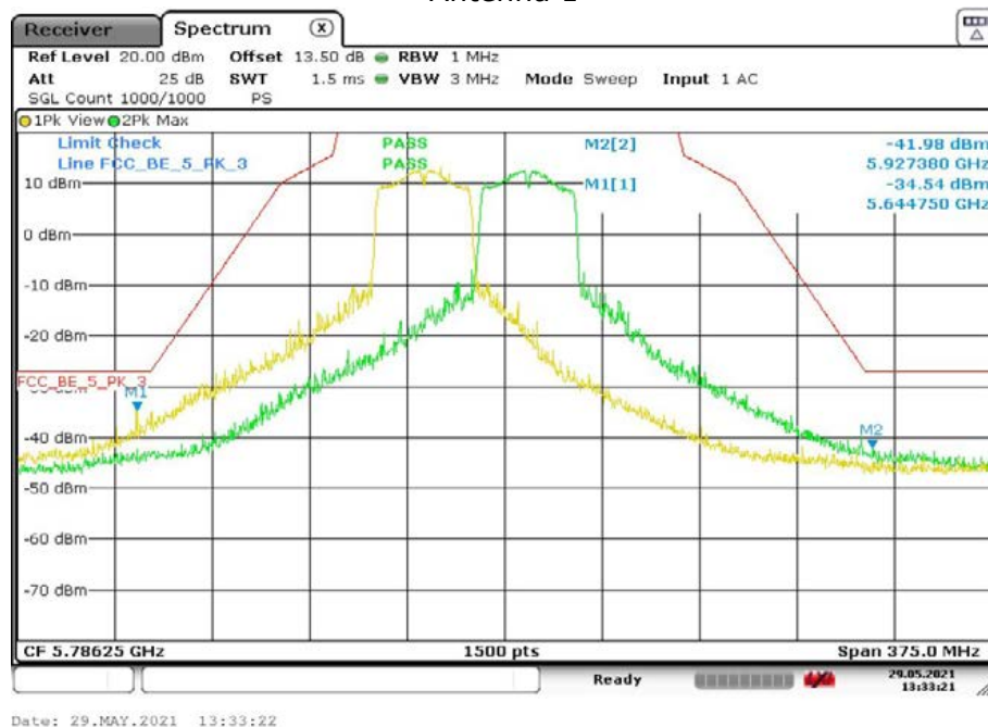
Antenna 1
