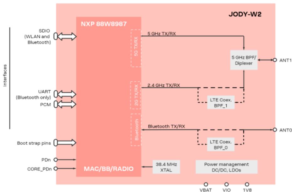
Internal Block Diagram
