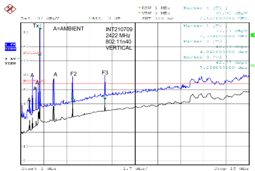
2422 MHz–Peak/Average Vertical Polarisation
