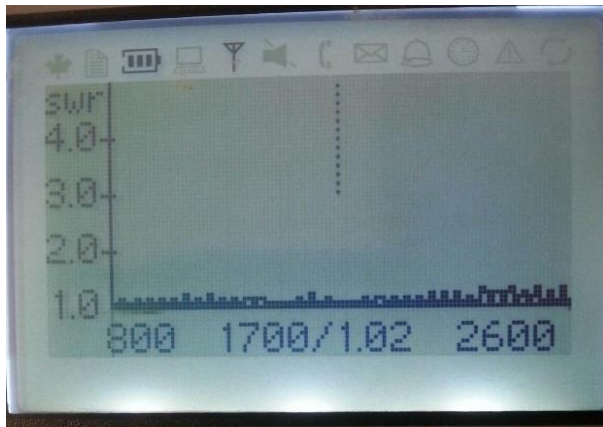
Good cable terminations
