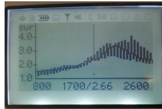
Poor cable terminations
