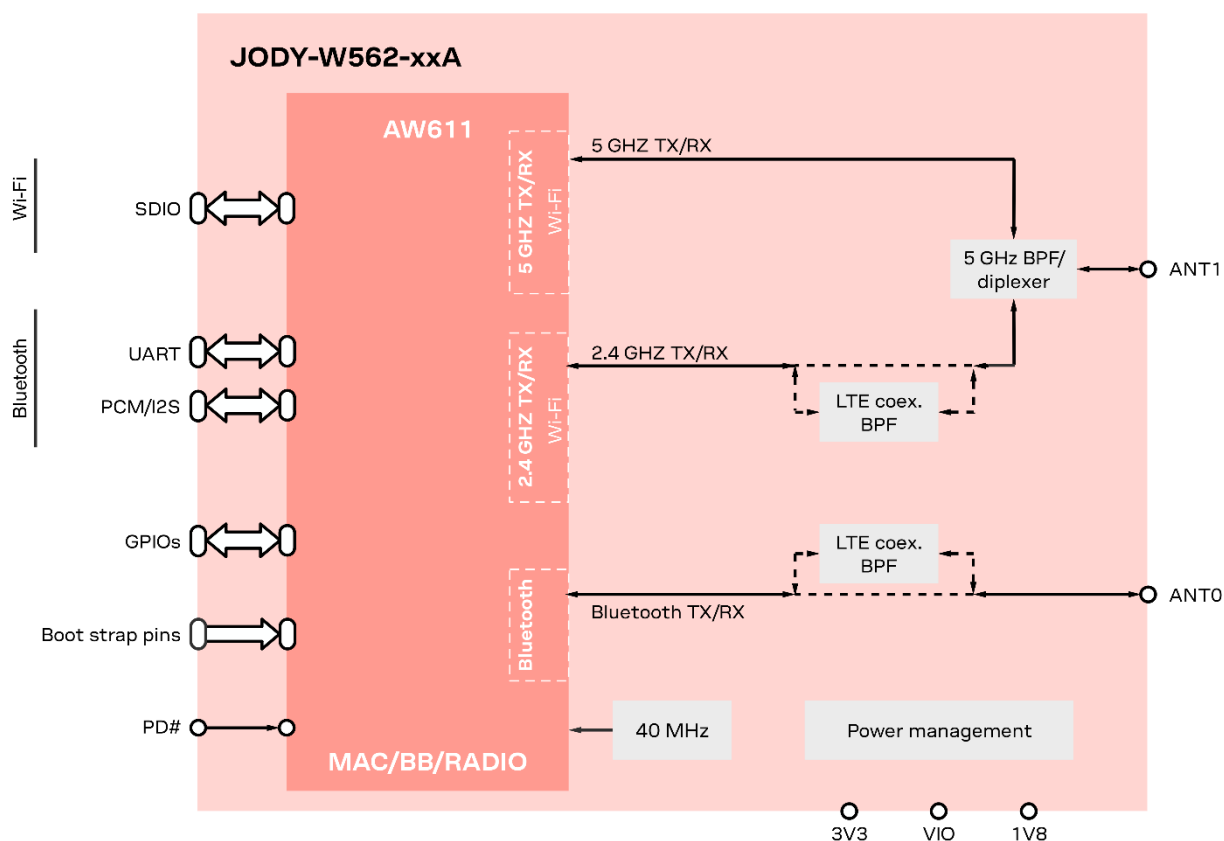
Figure 1: JODY-W562-xxA block diagram
