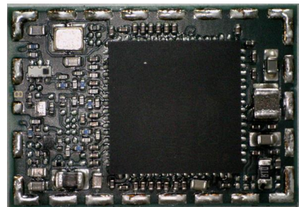
Figure 4: JODY-W562-21A module internal photo
