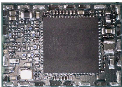
Figure 3: JODY-W562-01A module internal photo
