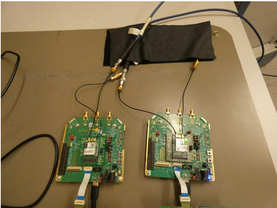
Photo 8: Test setup for DFS conducted measurement EUT detail
