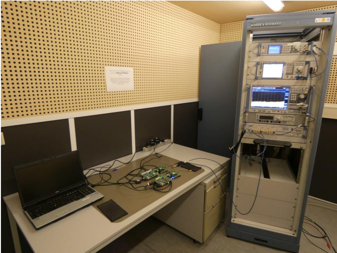
Photo 7: Test setup for DFS conducted measurements
