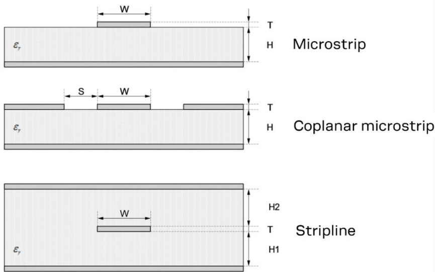
Figure 5: Transmission line trace design
