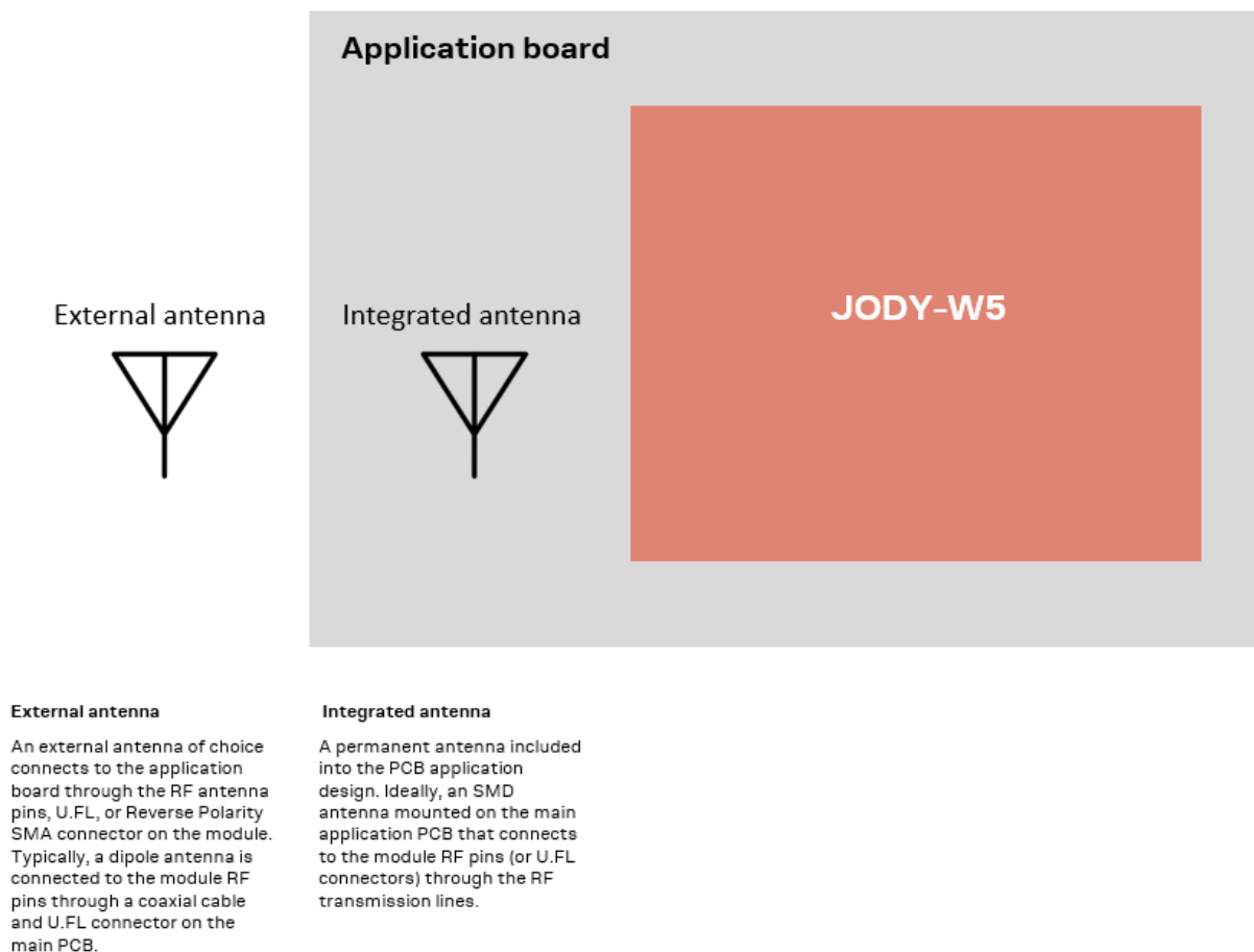
Figure 3: Antenna options
