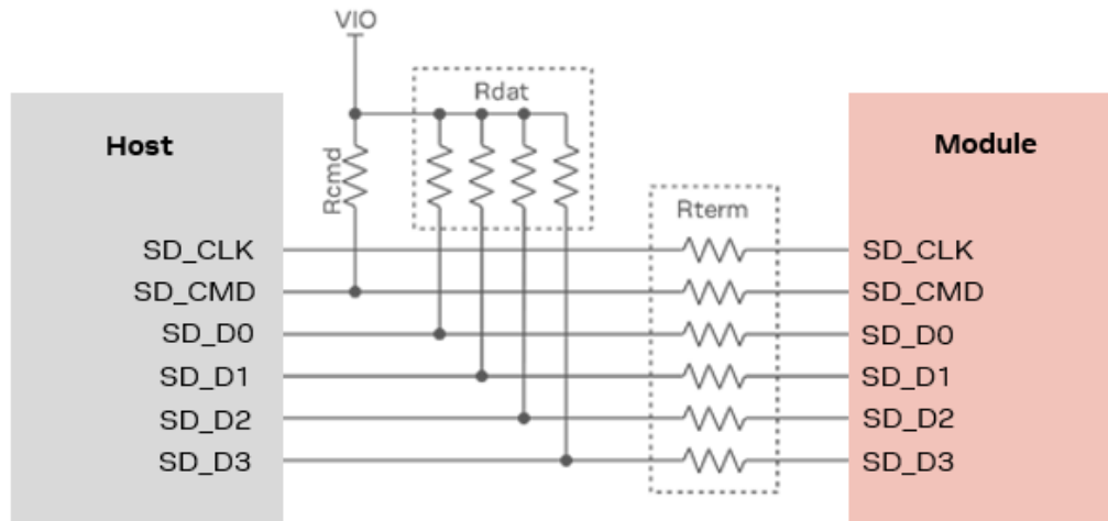
Figure 9: SDIO application schematic
