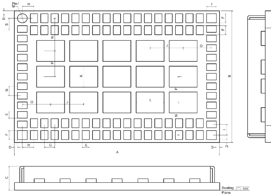
Figure 10: Recommended footprint for JODY-W5, bottom view
