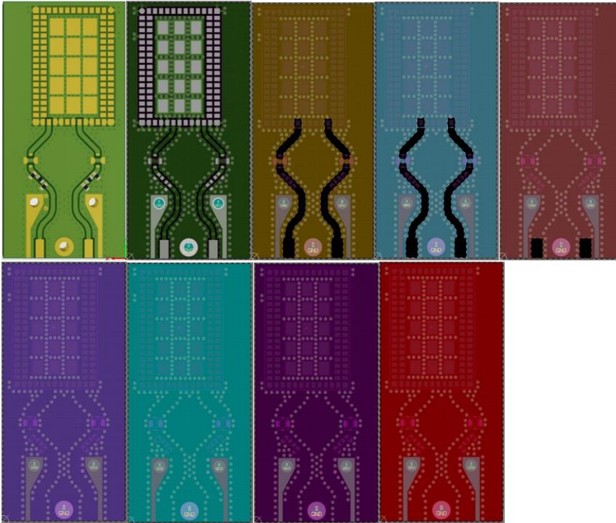
Figure 6: RF trace and ground design example
