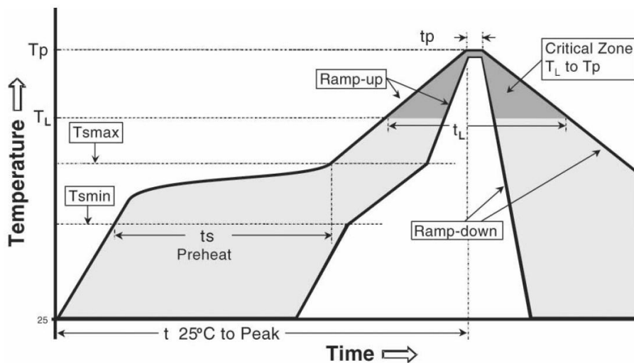
Figure 13: Reflow profile
