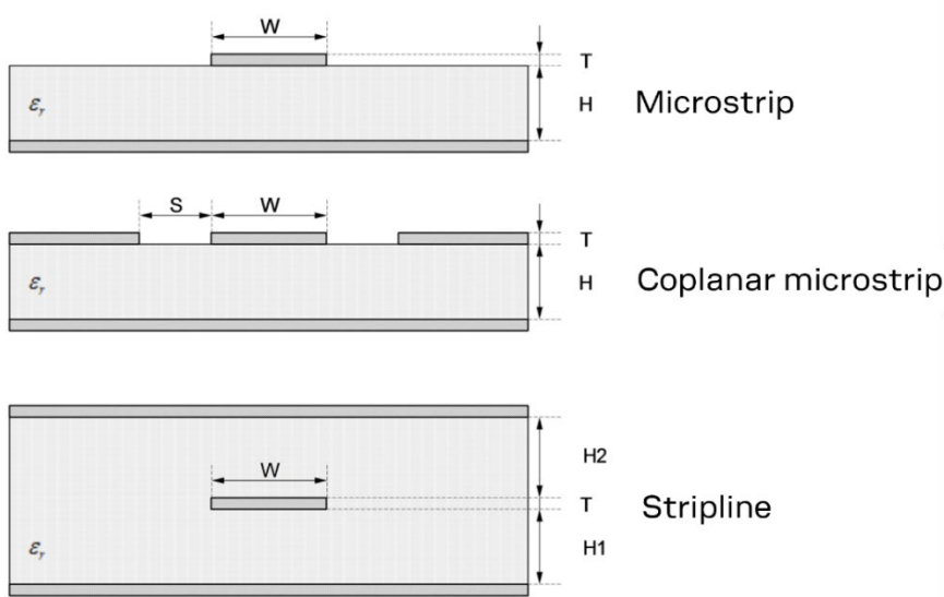
Figure 5: Transmission line trace design
