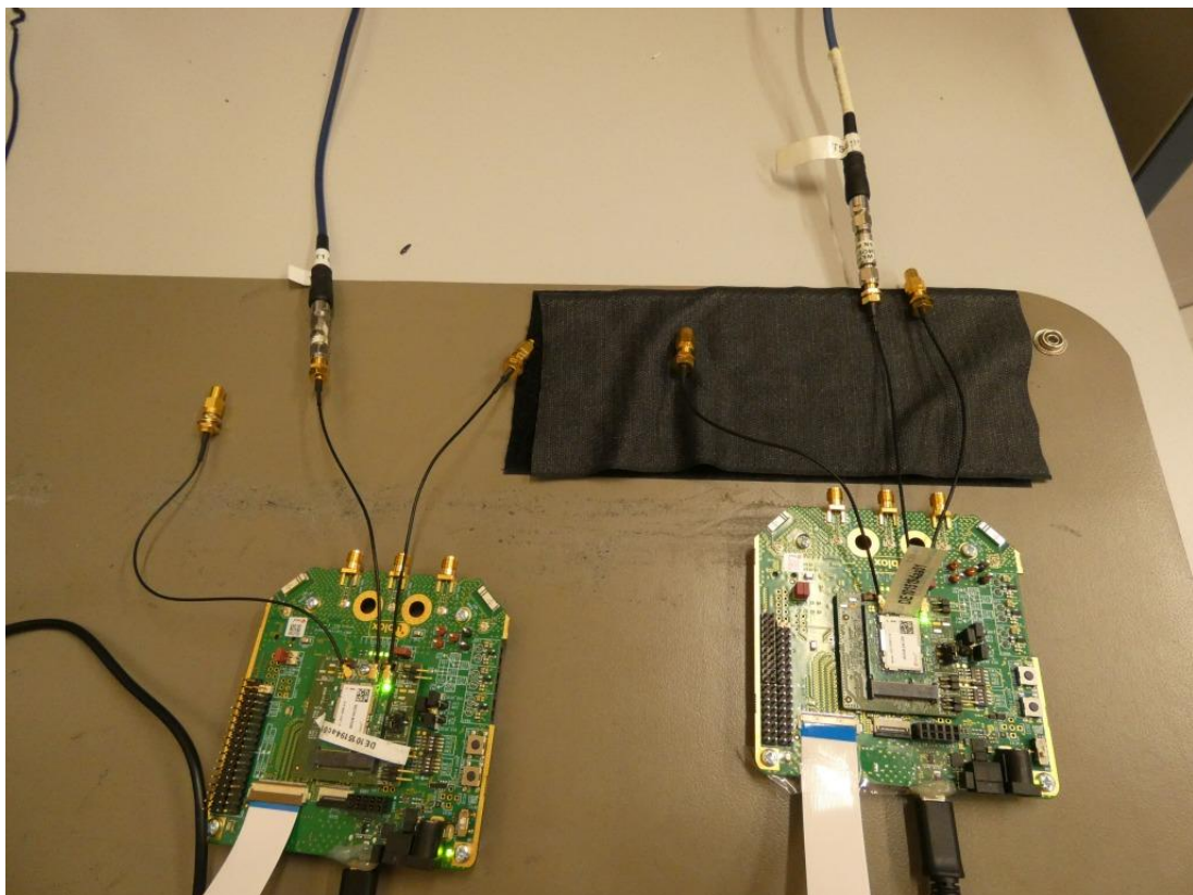
Photo 8: Test setup for DFS and Contention Based Protocol EUT detail
