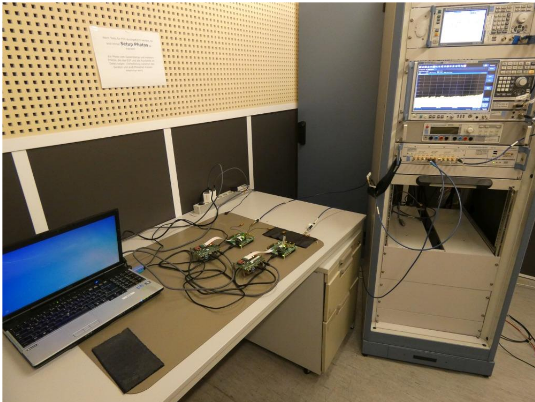
Photo 7: Test setup for DFS and Contention Based Protocol
