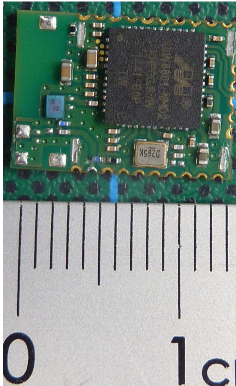
160785_m.jpg: Lily-W131 module without shielding – top view
