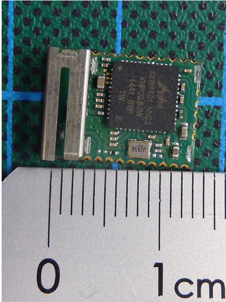
160785_n.jpg: Lily-W132 module without shielding – top view
