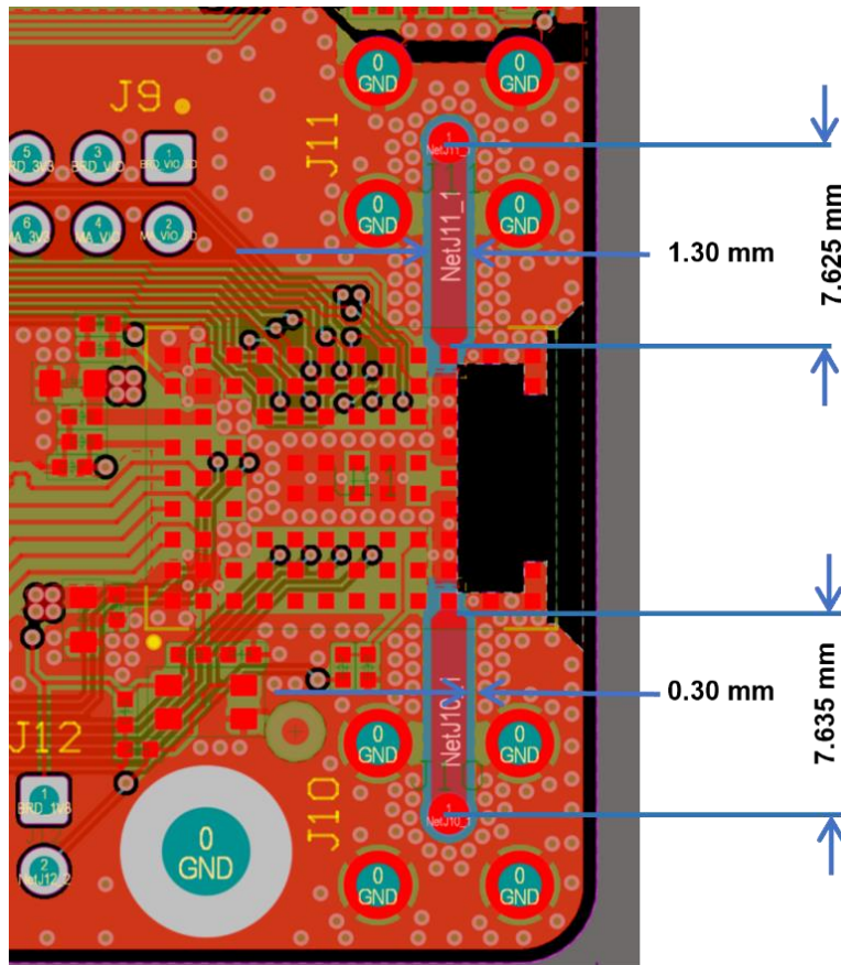
Figure 3: Evaluation board artwork with dimensions
