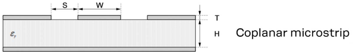
Figure 2: Coplanar microstrip structure
