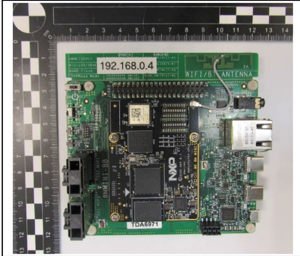
Evaluation board top view
