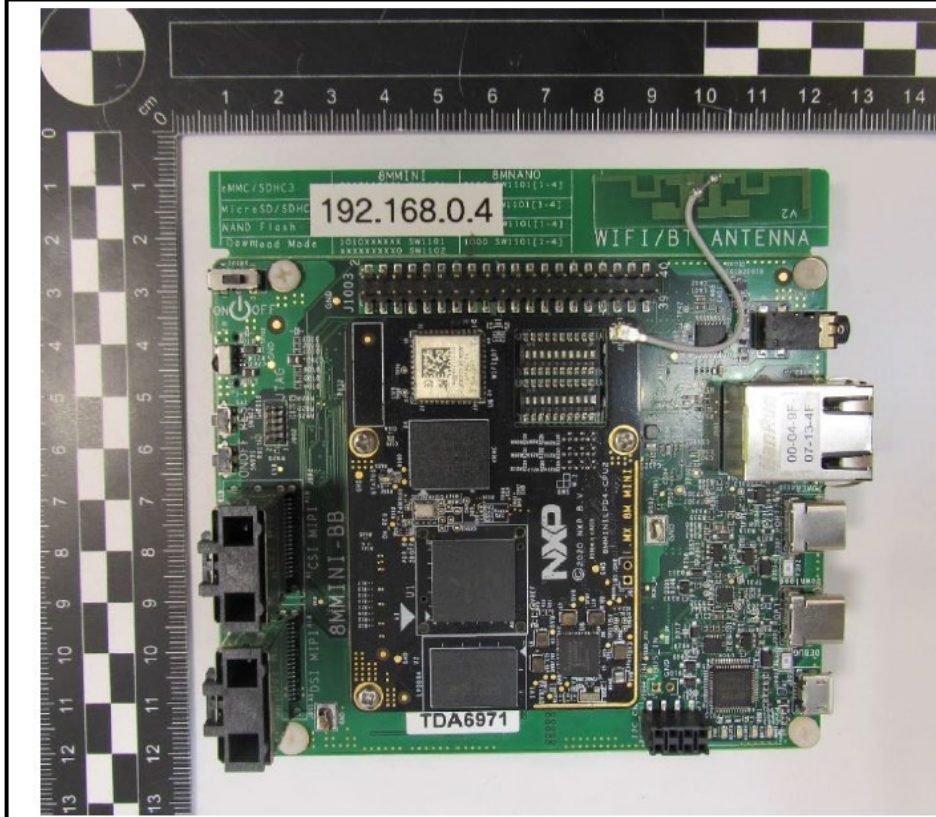
Evaluation board top view
