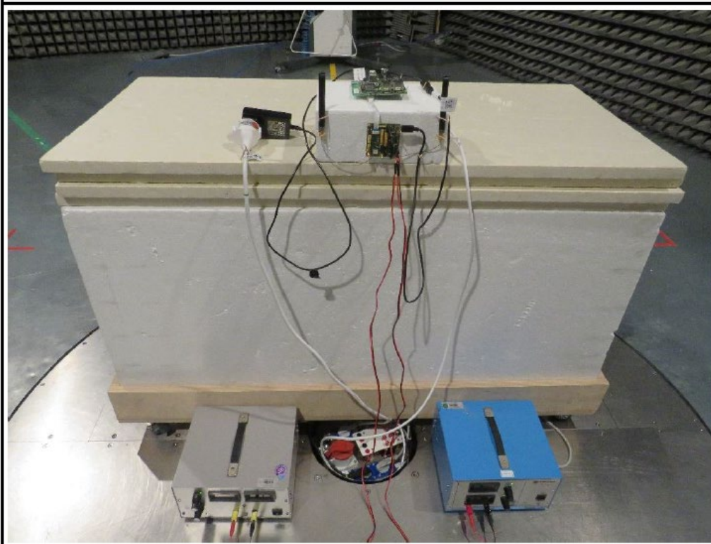
EUT Test Setup below 1 GHz
