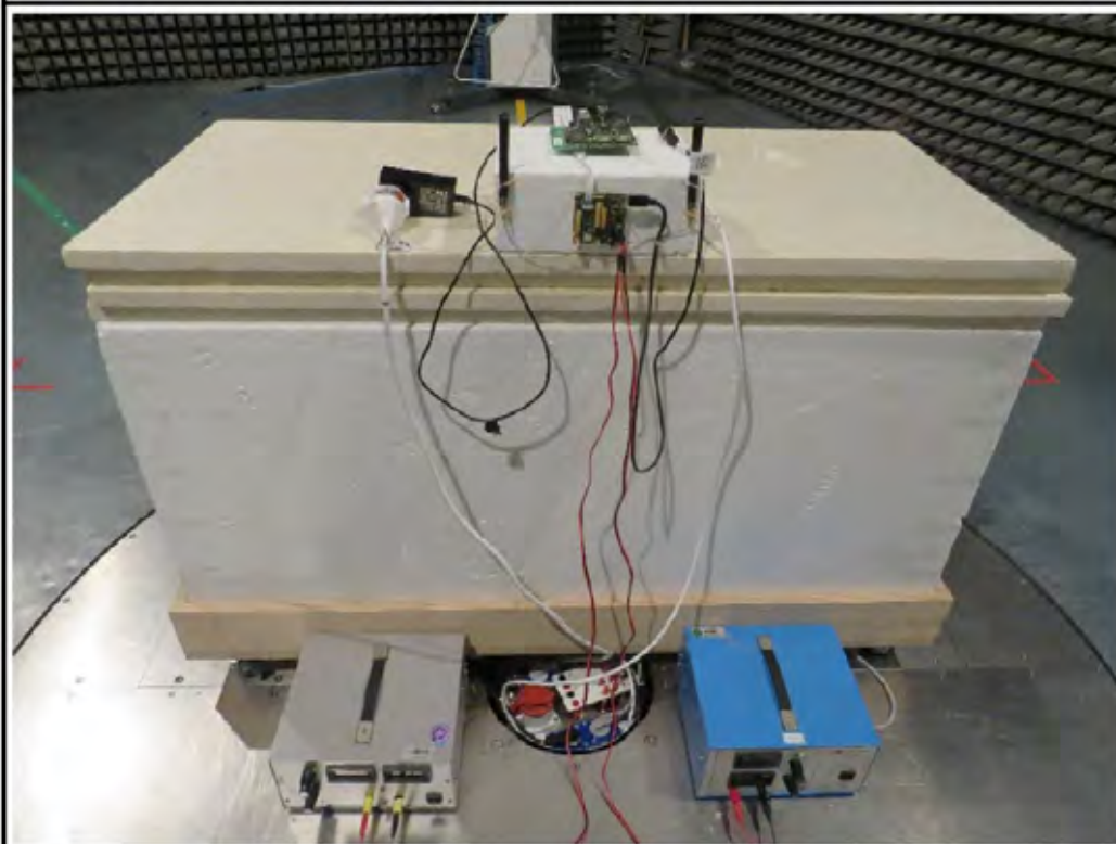
EUT Test Setup below 1 GHz
