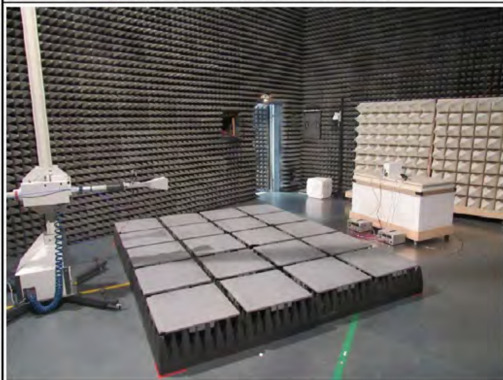
Setup for measurements above 1 GHz (1)
