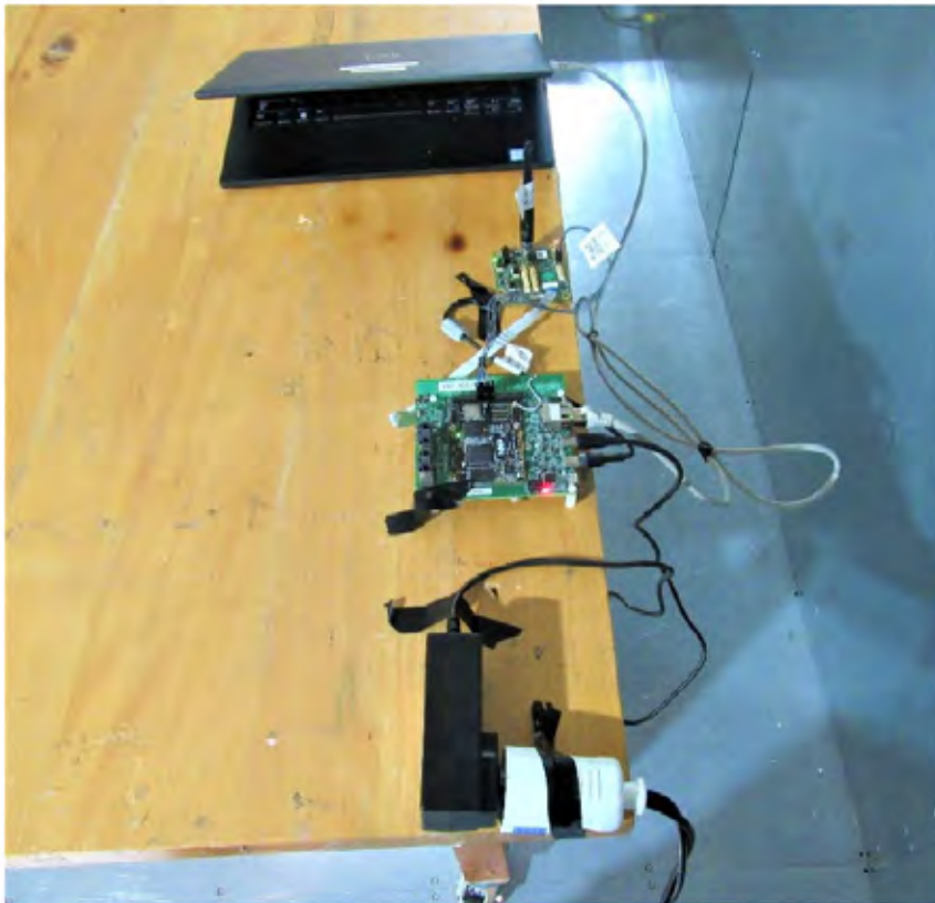
Setup for measurements 150 KHz - 30 MHz (Cables)
