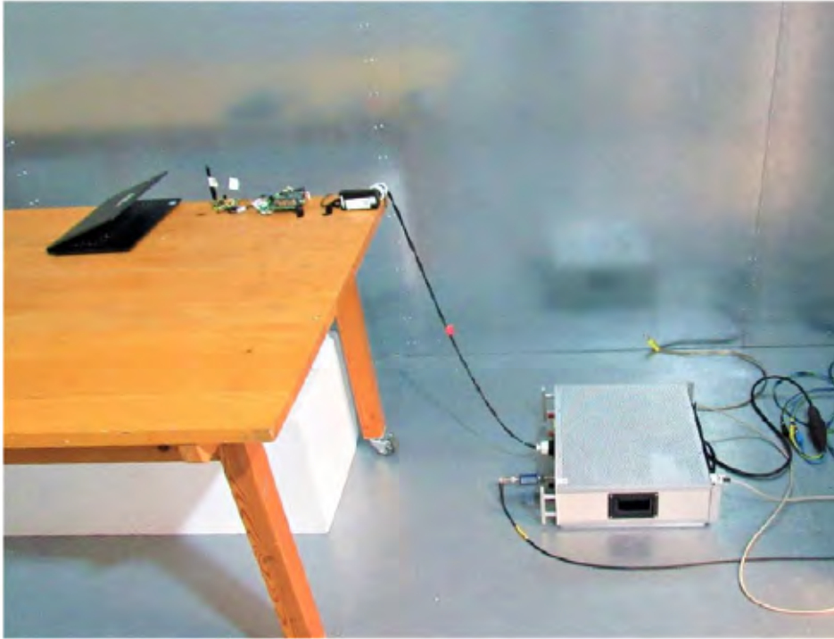
Setup for measurements 150 KHz - 30 MHz
