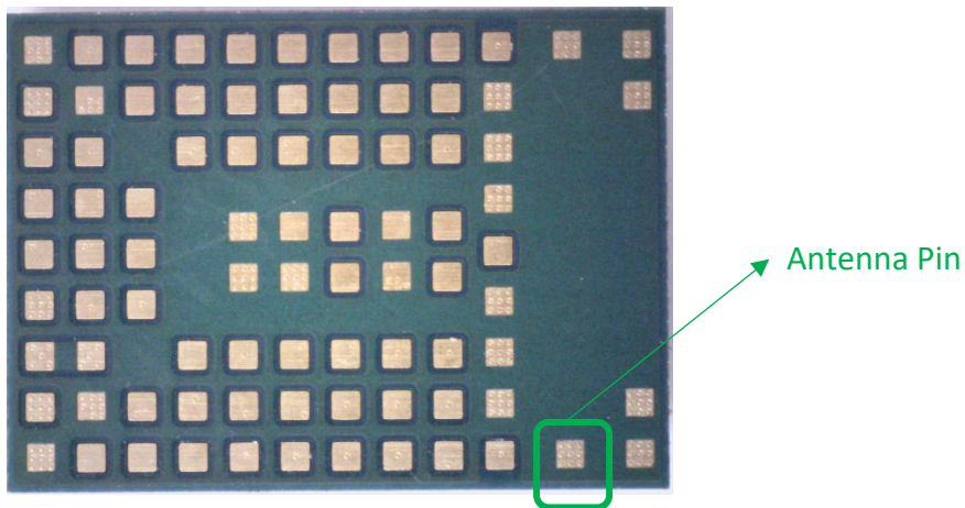
Figure 3: Bottom view of MAYA-W276-00B and MAYA-W266-00B
