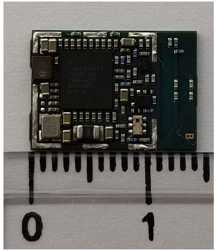
Figure 9: MAYA-W266-00B length 14.3mm (internal photo)
