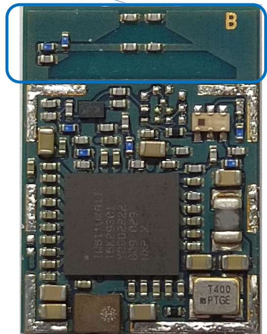
Figure 5: MAYA-W266-00B top view internal photo
