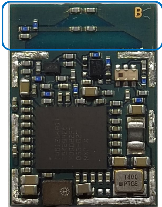
Figure 4: MAYA-W276-00B top view internal photo
