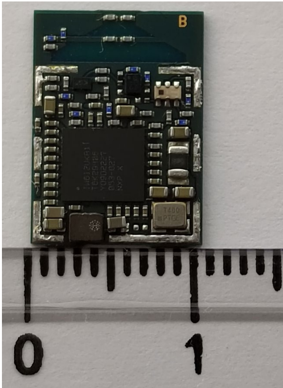
Figure 8: MAYA-W266-00B width 10.4 mm (internal photo)
