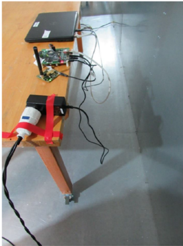
Setup for measurements 150 kHz - 30 MHz (cables)
