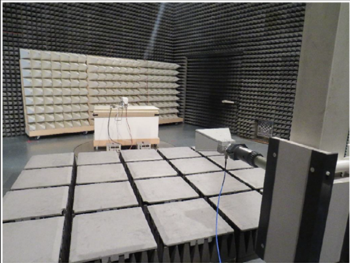
Setup for measurements above 1 GHz
