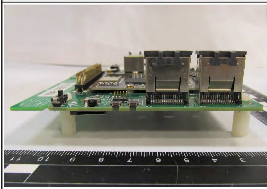
Evaluation board side view
