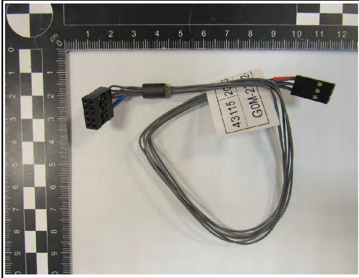
Cable (SPI Cable)
