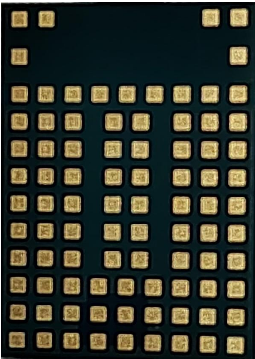
Figure 2: Bottom view of MAYA-W362-00B
