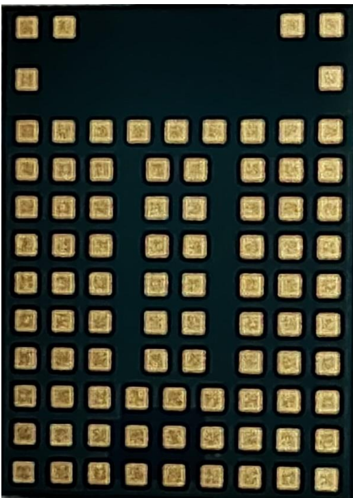
Figure 2: Bottom view of MAYA-W361-00B
