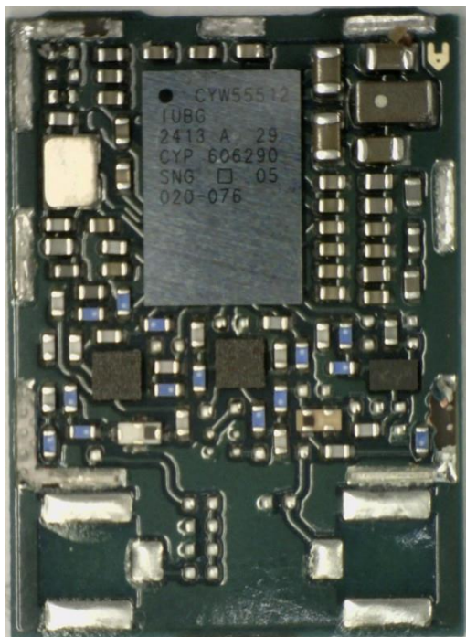
Figure 1: MAYA-W361-00B internal photo
