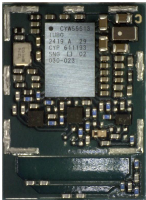
Figure 1: MAYA-W386-00B internal photo
