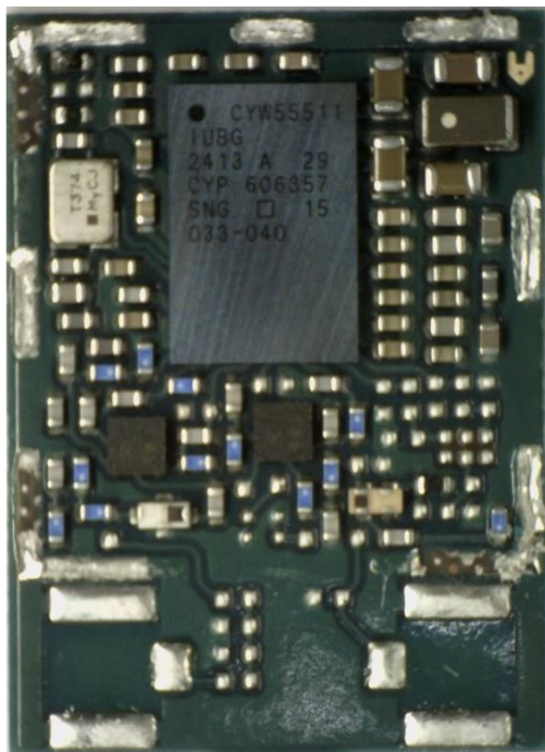
Figure 1: MAYA-W331-00B internal photo
