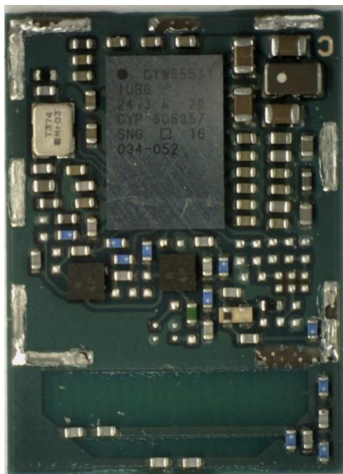
Figure 1: MAYA-W336-00B internal photo
