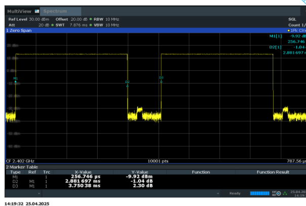
Bluetooth BDR DH5
