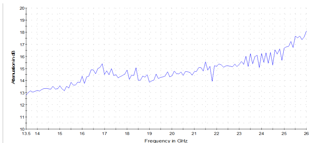
Transducer DUT1_3dB_HF11
