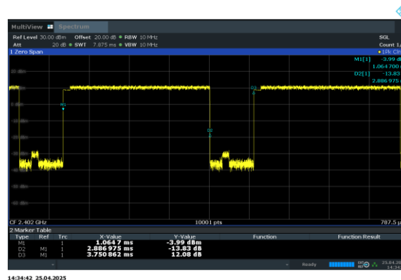
Bluetooth EDR3 3-DH5
