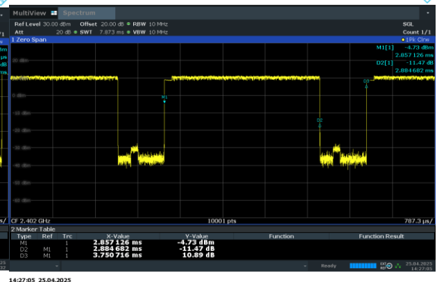
Bluetooth EDR2 2-DH5
