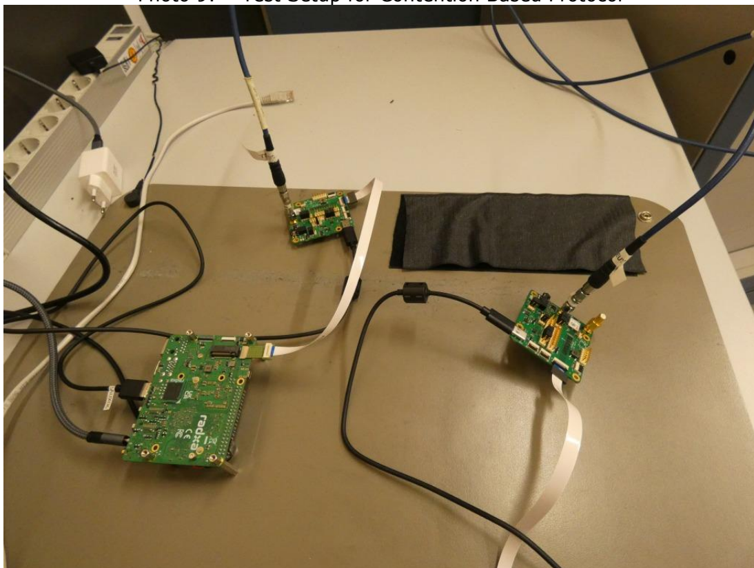
Photo 10: Test Setup for Contention Based Protocol EUT Detail
