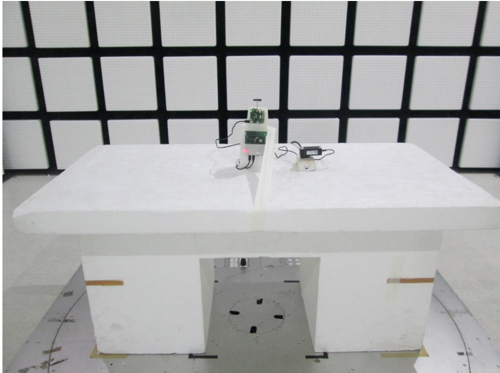
MAYA-W473-10B PCB Antenna
