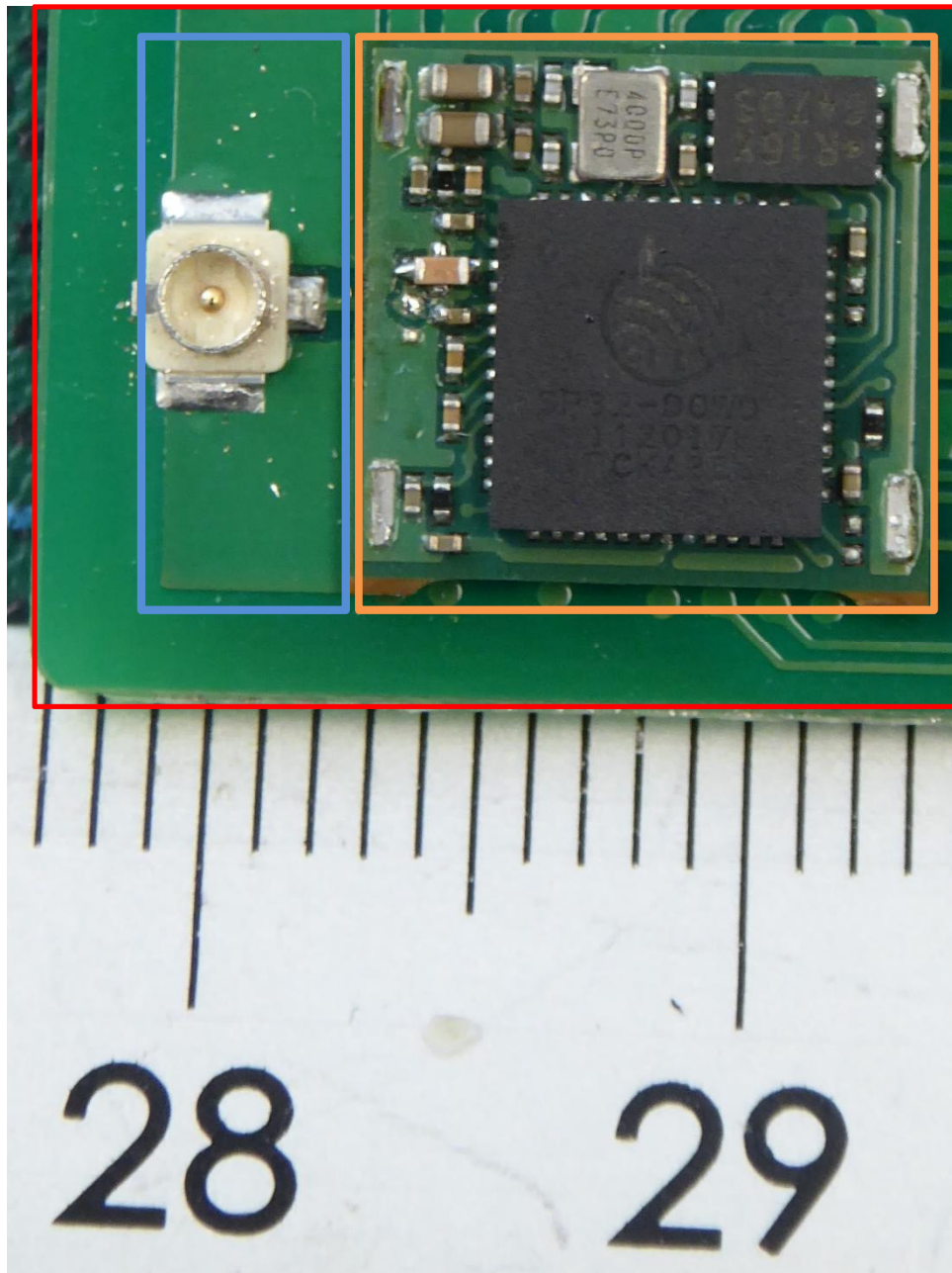
170297_E8_20.jpg: EUT with antenna trace design on not marketed eval board – without shielding
