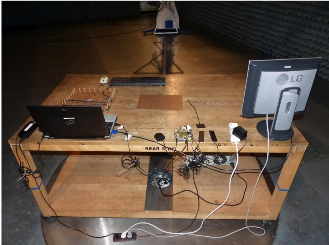
Photo 2: Test setup AE02 for radiated measurements, unintentional radiator §15) single device setup, computer peripheral.
