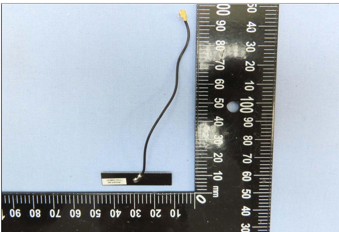
Antenna (Brand: WNC, Model: BB-8)
