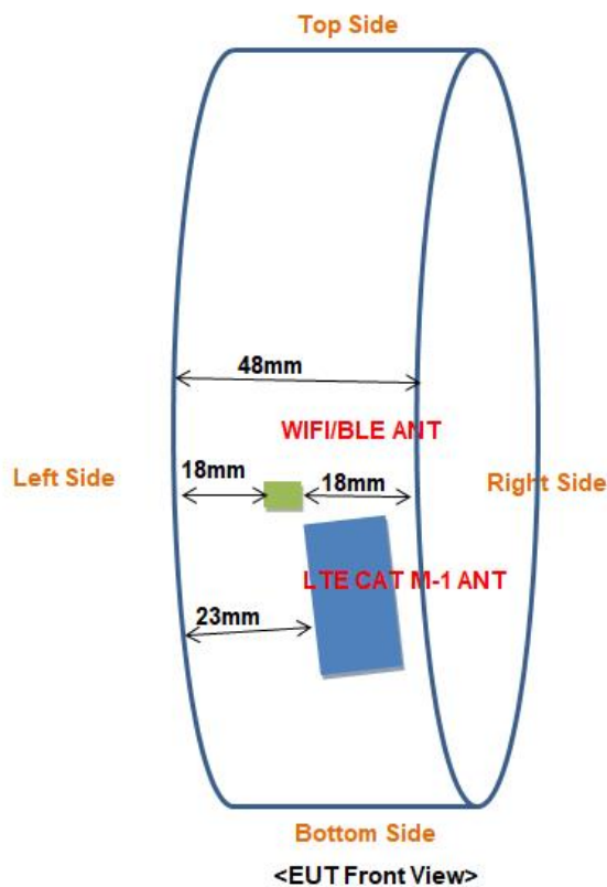
Block Diagram for EUT Antenna Position
