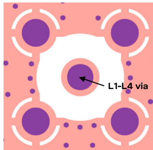
Figure 39: 50 \Omega SMA female connector layout on the u-blox host PCB
