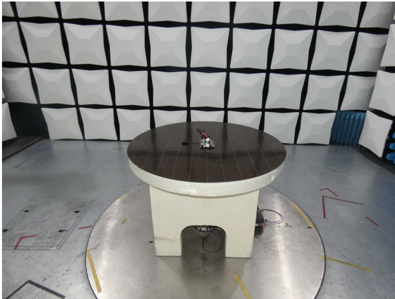
Photo 4: Test setup for radiated measurements below 1GHz
