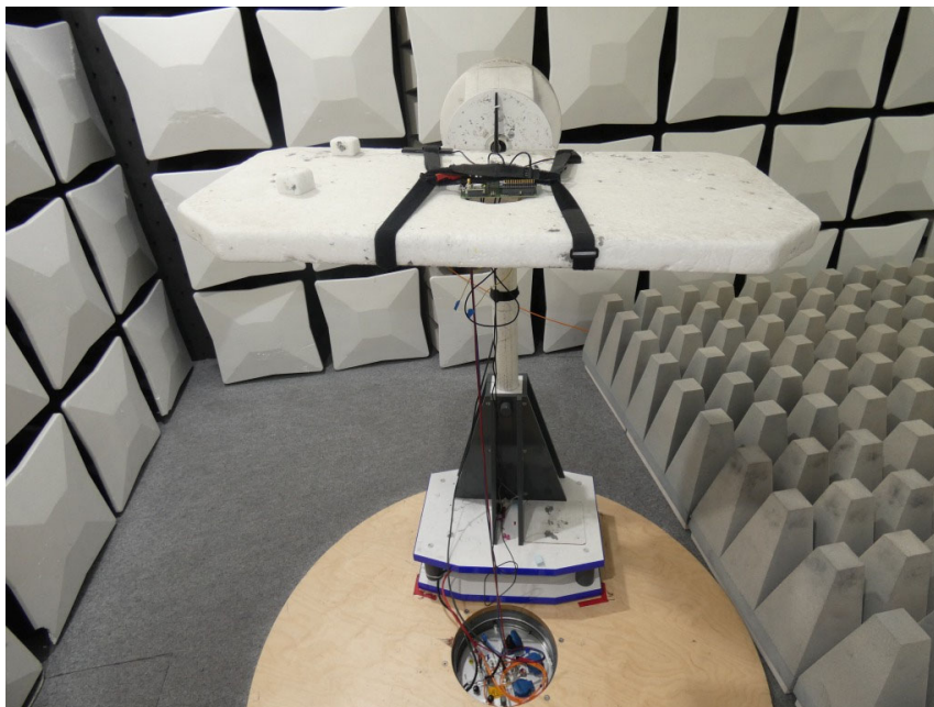
Photo 1: Test setup for radiated measurements above 1GHz
