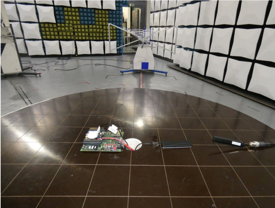
Photo 6: Test Antenna
