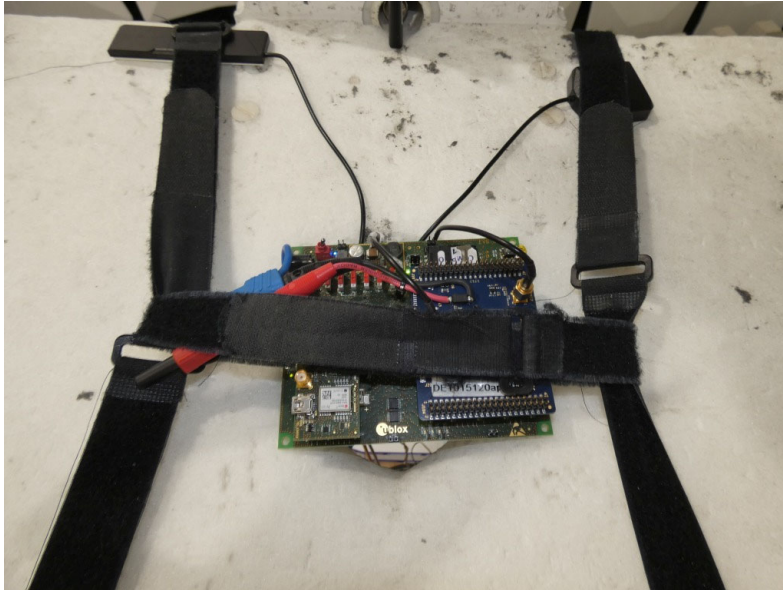
Photo 2: EUT setup
