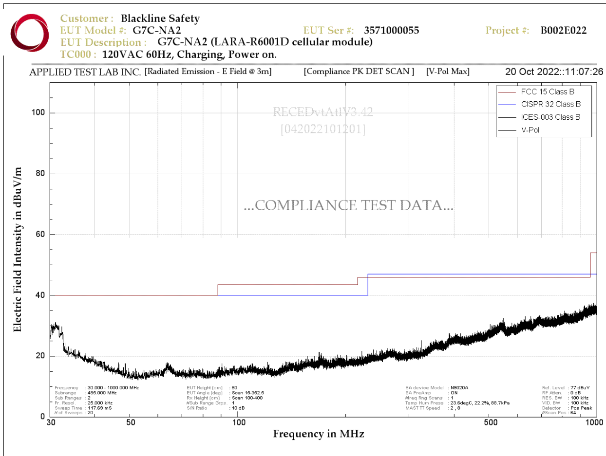
Figure 6.4 - Radiated Emission (FCC and ICES-003) - Scan Vertical Polarization (30MHz - 1000MHz)
