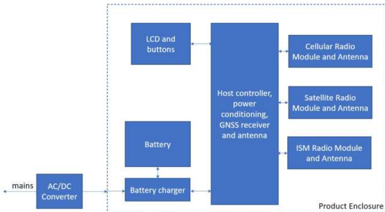
EUT functional setup Diagram
