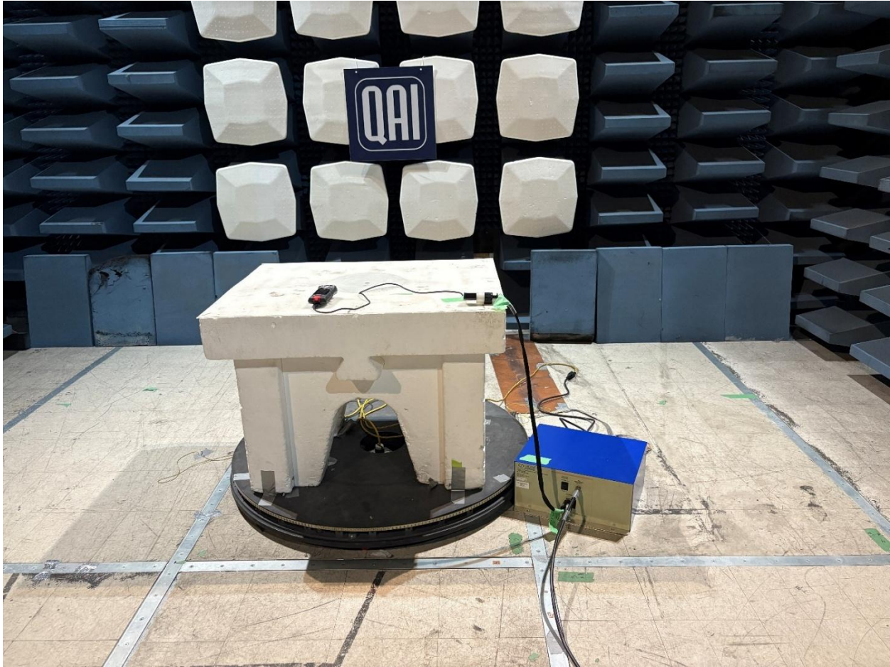
Figure 4: AC Mains Conducted Emissions – 150kHz to 30MHz
