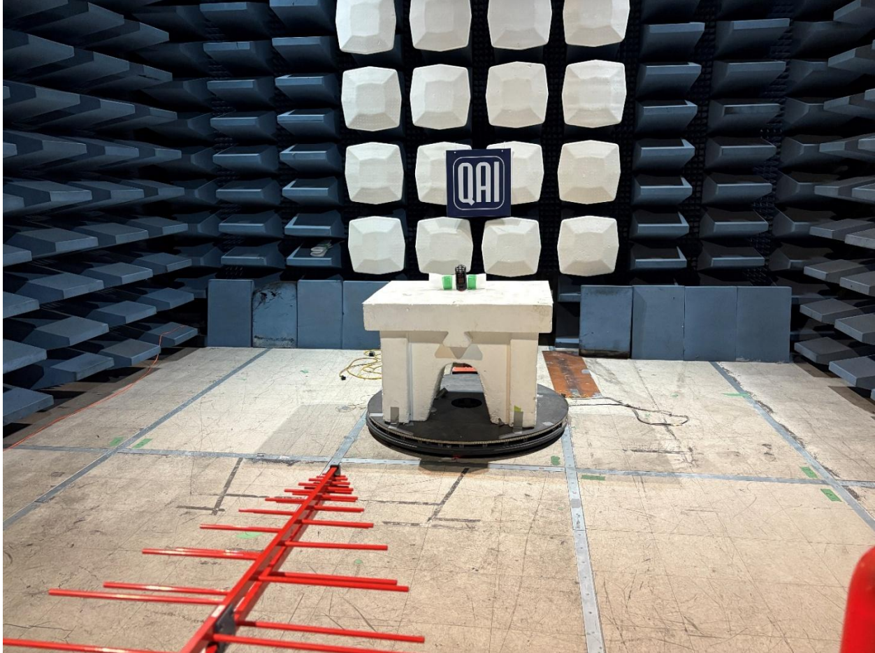
Figure 1: Radiated Emissions – 30MHz to 1GHz
