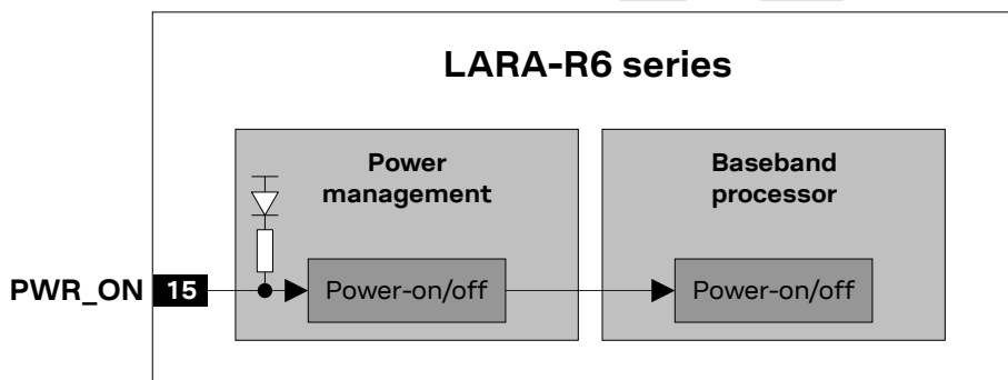
Figure 12: LARA-R6 series PWR_ON input description
