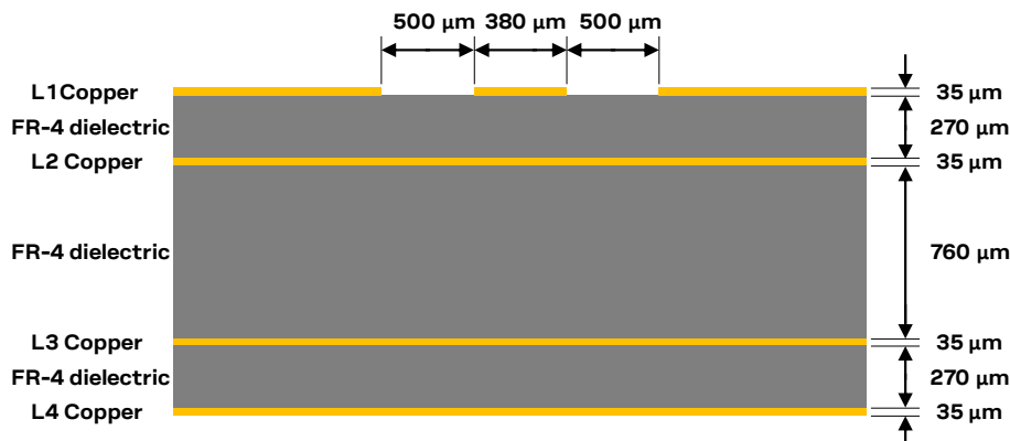
Figure 33: Example of a 50\ \Omega coplanar waveguide transmission line design for the described 4-layer board layout
