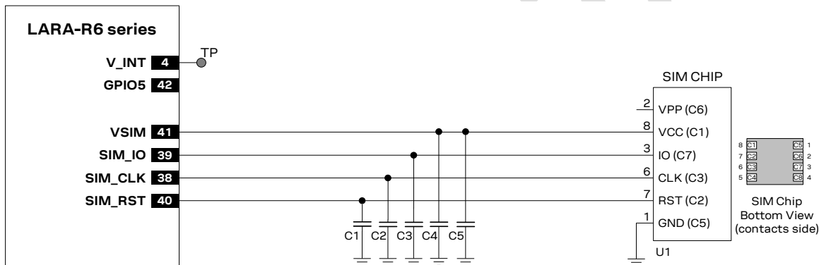
Figure 39: Application circuit for the connection to a single solderable SIM chip, with SIM detection not implemented
