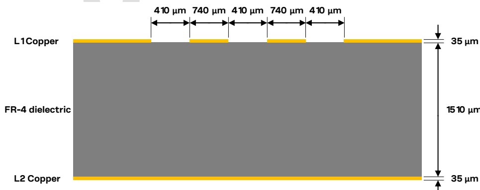
Figure 54: Example of USB line design, with Z_0 close to 90 \Omega and Z_{CM} close to 30 \Omega , for the described 2-layer board layup
