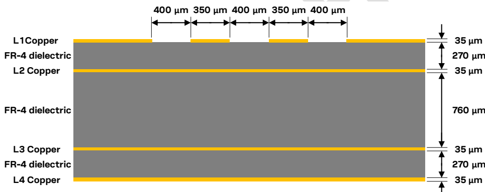
Figure 53: Example of USB line design, with Z_0 close to 90 \Omega and Z_{CM} close to 30 \Omega , for the described 4-layer board layup
