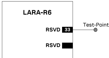
Figure 60: Application circuit for the reserved pins (RSVD)
