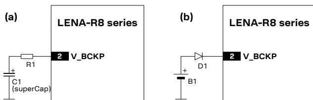
Figure 30: LENA-R8 series cellular system Real Time Clock supply (V_BCKP) application circuits
