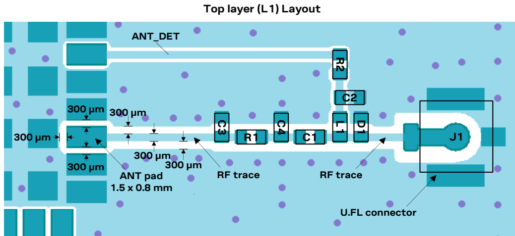
Figure 39: Top layer layout of the u-blox host PCB with the antenna trace design, and additional antenna detection circuit
