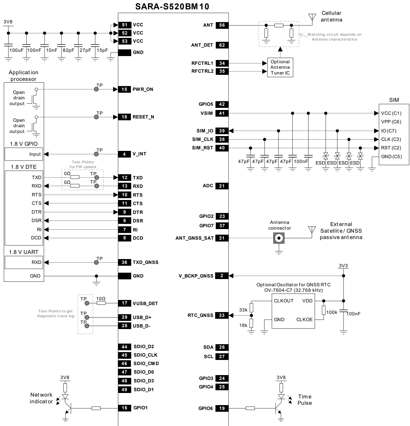
Figure 70: Example schematic diagram integrating a SARA-S520BM10 module
