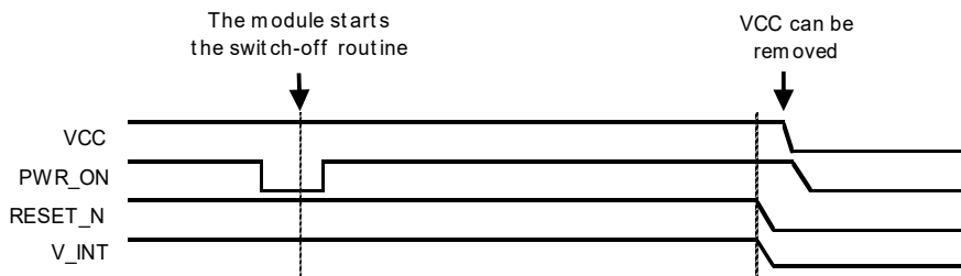
Figure 14: SARA-S520BM10 switch-off sequence by toggling the PWR_ON input pin
