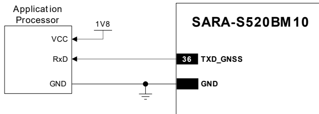
Figure 66: Application circuit for GNSS peripheral UART data output pin
