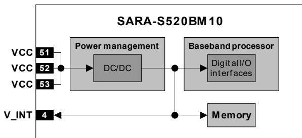
Figure 9: SARA-S520BM10 interfaces supply output (V_INT) simplified block diagram
