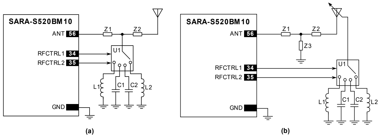
Figure 43: Examples of schematics for cellular antenna dynamic impedance tuning (a) and aperture tuning (b).
