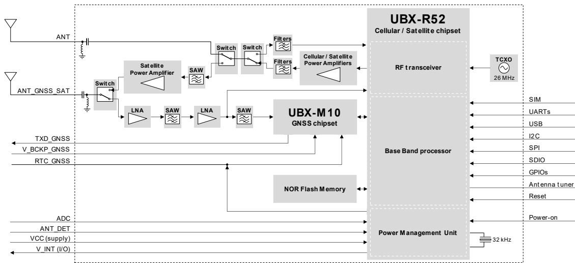
Figure 1: SARA-S520BM10 module simplified block diagram
