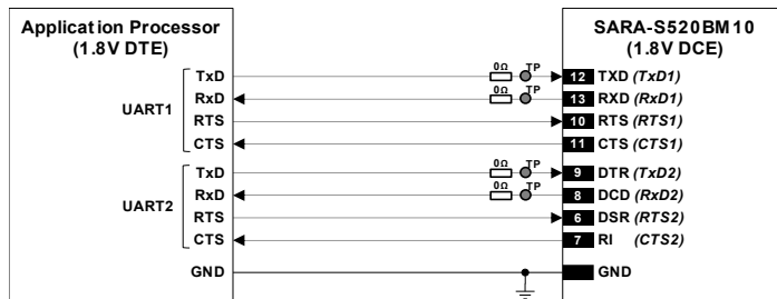
Figure 57: 2 UART interfaces application circuit with 5-wire links in DTE/DCE serial communications (1.8 V DTE)
