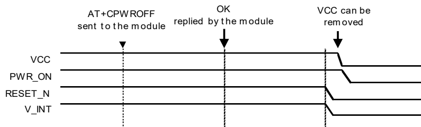
Figure 13: SARA-S520BM10 switch-off sequence by the +CPWROFF AT command
