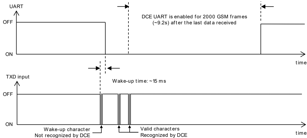
Figure 19: Wake-up via data reception with further communication
