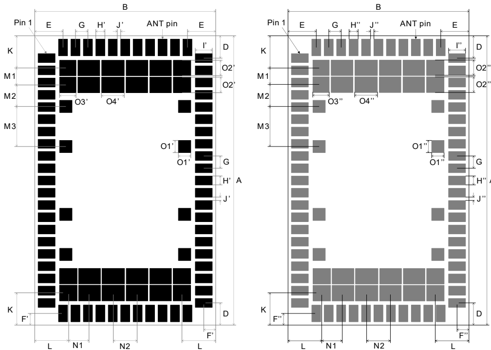
Figure 69: SARA-S520BM10 suggested footprint and paste mask (application board top view)
