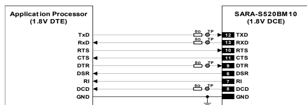
Figure 51: 1 UART interface application circuit with complete V.24 link in DTE/DCE serial communication (1.8 V DTE)
