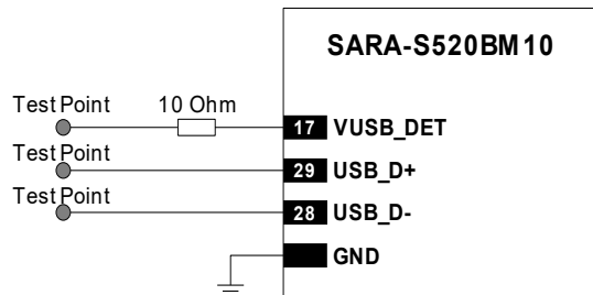
Figure 63: SARA-S520BM10 USB application circuit providing access for diagnostic purposes
