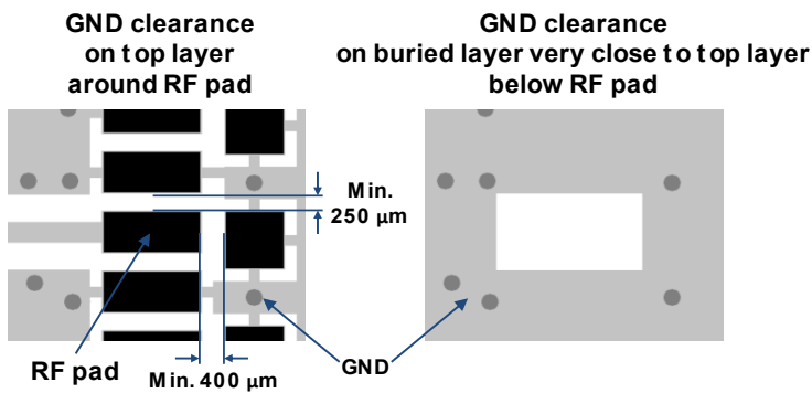
Figure 33: GND keep-out area on top layer around RF pad and on closely buried layer below RF pad (ANT / ANT_GNSS_SAT)
