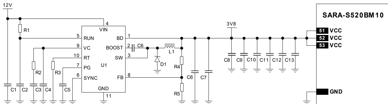
Figure 21: Example of VCC supply circuit for SARA-S520BM10, using a step-down regulator
