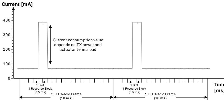
Figure 6: VCC current consumption profile during LTE Cat M1 half-duplex connection
