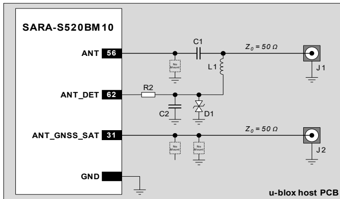
Figure 44: Antenna trace design implemented on the host PCB, with additional antenna detection circuit
