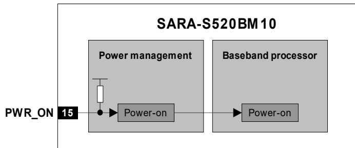
Figure 10: SARA-S520BM10 PWR_ON input equivalent circuit description
