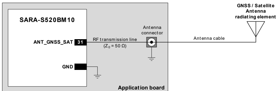
Figure 38: Minimum circuit with GNSS / Satellite passive antenna
