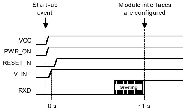
Figure 11: SARA-S520BM10 switch-on sequence description from not-powered mode
