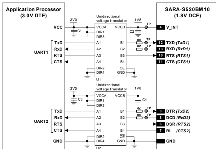
Figure 58: 2 UART interfaces application circuit with 5-wire links in DTE/DCE serial communications (3.0 V DTE)
