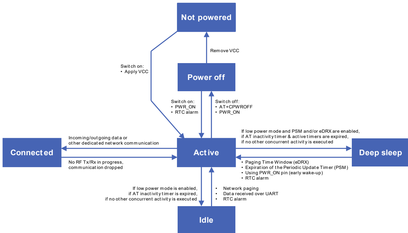
Figure 3: SARA-S520BM10 operating mode transitions with cellular LTE Cat M1 RAT enabled
