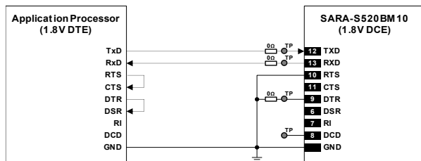
Figure 59: 1 UART interface application circuit with 3-wire link in DTE/DCE serial communication (1.8 V DTE)
