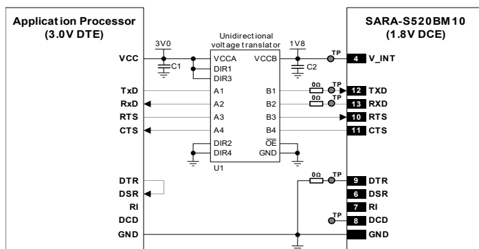
Figure 56: 1 UART interface application circuit with 5-wire link in DTE/DCE serial communication (3.0 V DTE)
