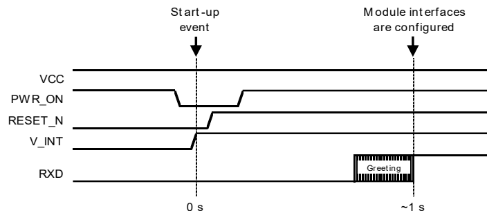
Figure 12: SARA-S520BM10 switch-on / early wake-up sequence description from power-off / deep-sleep mode
