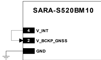
Figure 30: V_BCKP_GNSS application circuit shorting with V_INT supply
