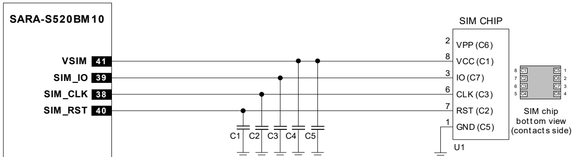
Figure 49: Application circuits for the connection to a single Surface-Mounted SIM chip
