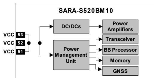
Figure 4: SARA-S520BM10 illustrative internal VCC supply routing
