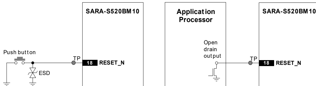
Figure 32: RESET_N application circuits using a push button and an open drain output of an application processor
