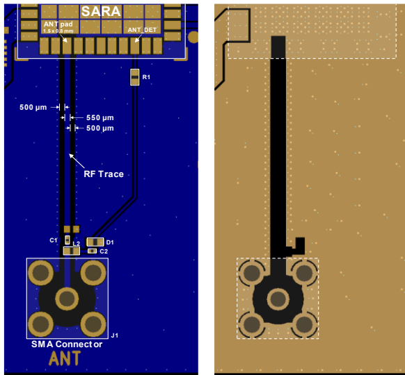
Figure 45: Top layer (L1) and buried layer (L2) layout of the host PCB with the Cellular antenna RF trace design
