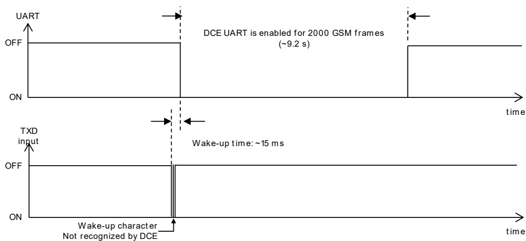
Figure 18: Wake-up via data reception without further communication
