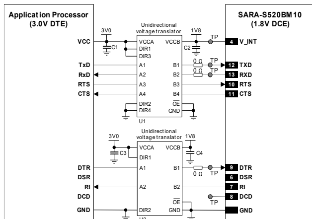
Figure 54: 1 UART interface application circuit with 7-wire link in DTE/DCE serial communication (3.0 V DTE)
