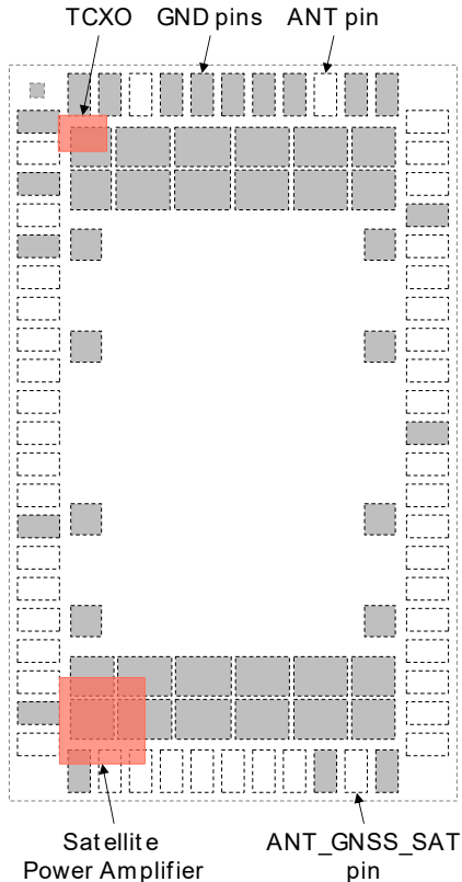
Figure 28: TCXO, Satellite PA, GND and RF pins location on SARA-S520BM10 (top view / module through view)
