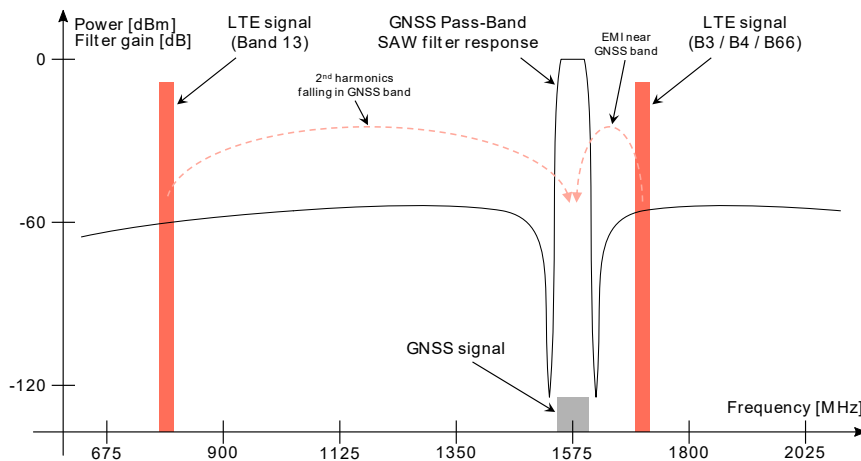
Figure 39: EMI due to Tx in LTE B3, B4, B66 low channels (1710 MHz) adjacent to GNSS frequency range (1559 to 1610 MHz), or due to Tx in LTE B13 high channels (787 MHz) with harmonics falling into the GNSS frequency range
