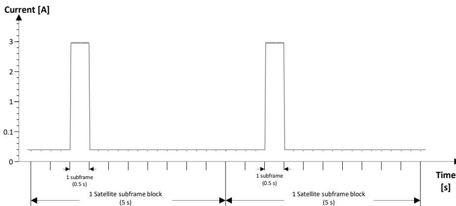
Figure 5: VCC current consumption profile during satellite transmission
