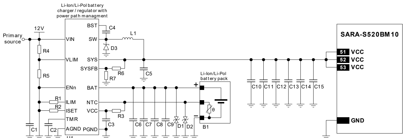
Figure 25: Li-Ion (or Li-Pol) battery charging and power path management application circuit
