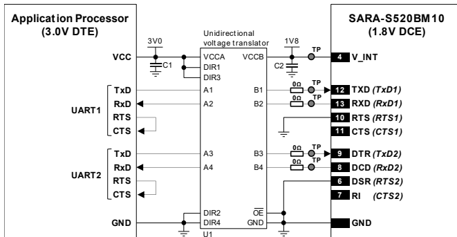
Figure 62: 2 UART interfaces application circuit with 3-wire links in DTE/DCE serial communications (3.0 V DTE)
