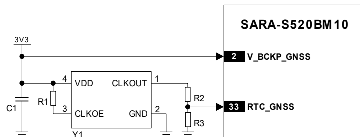
Figure 67: GNSS RTC application circuit with clock provided externally
