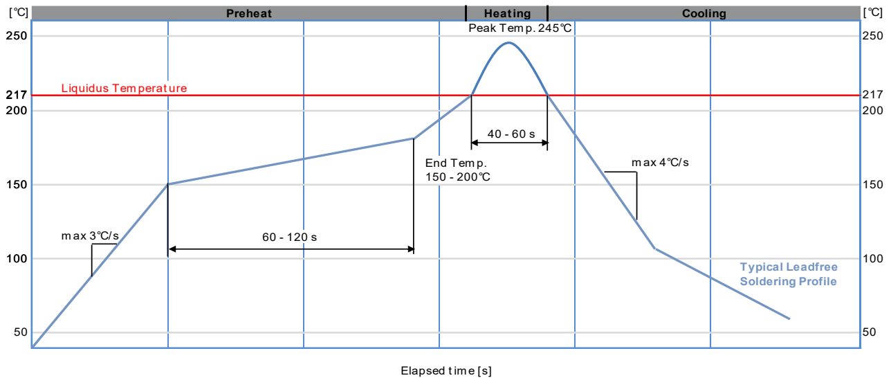
Figure 71: Recommended soldering profile
