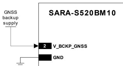
Figure 29: V_BCKP_GNSS application circuit using an independent power supply
