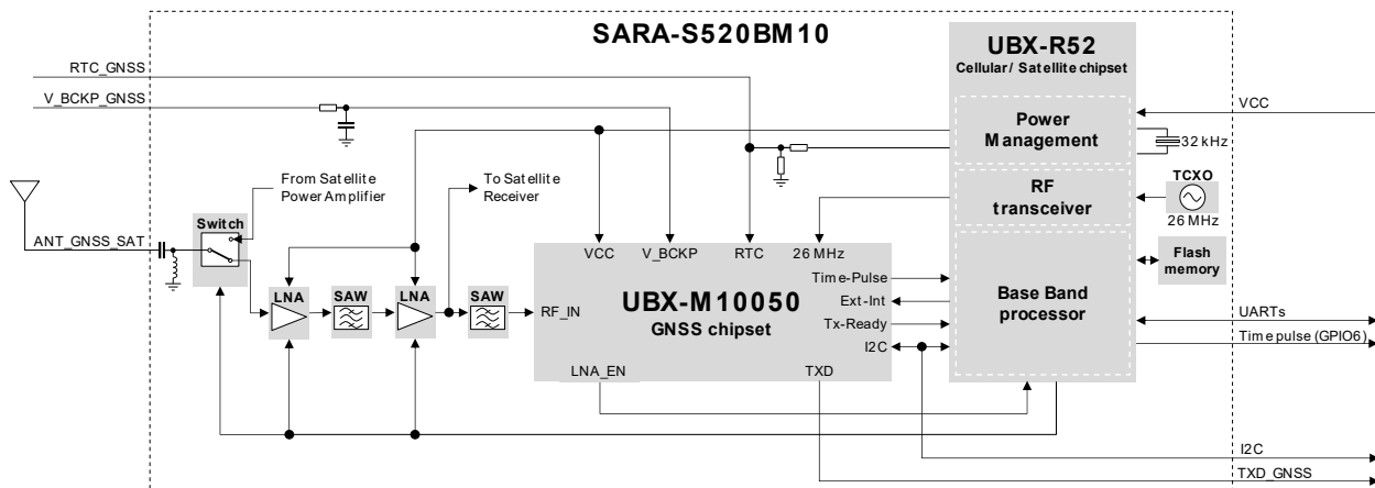
Figure 2: SARA-S520BM10 GNSS section block diagram
