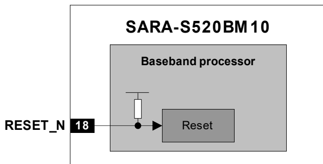
Figure 15: SARA-S520BM10 RESET_N input equivalent circuit description
