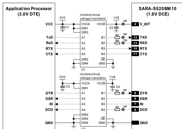
Figure 52: 1 UART interface application circuit with complete V.24 link in DTE/DCE serial communication (3.0 V DTE)
