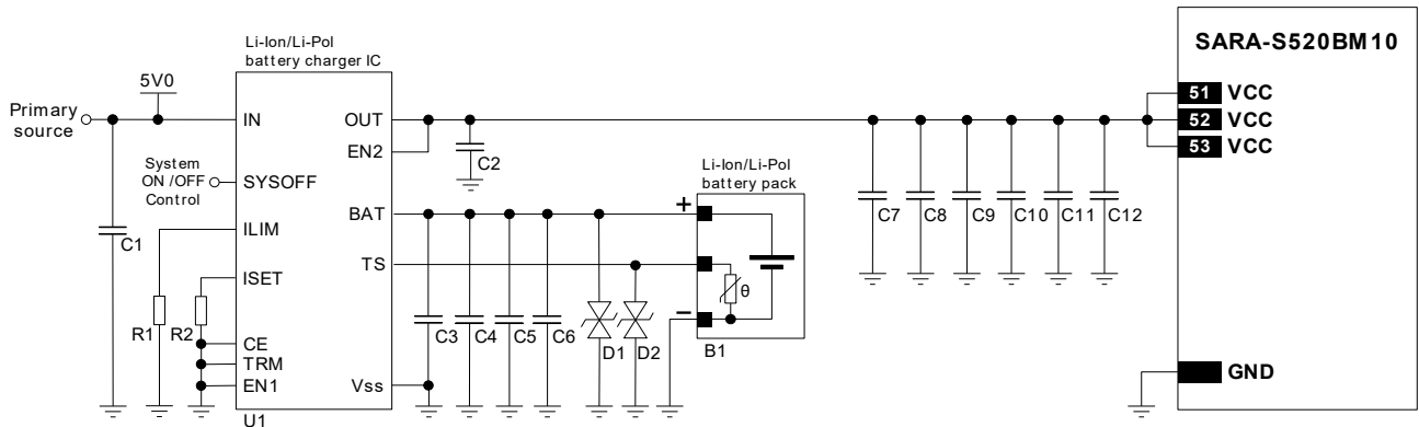
Figure 23: Li-Ion (or Li-Pol) battery charging application circuit
