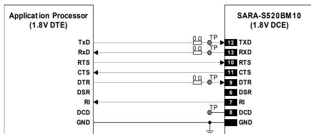
Figure 53: 1 UART interface application circuit with 7-wire link in DTE/DCE serial communication (1.8 V DTE)
