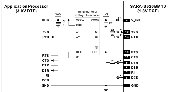
Figure 60: 1 UART interface application circuit with 3-wire link in DTE/DCE serial communication (3.0 V DTE)
