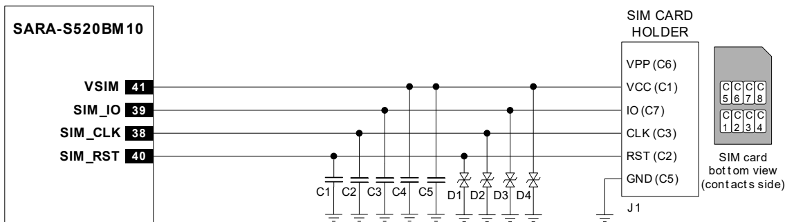
Figure 48: Application circuit for the connection to a single removable SIM card, with SIM detection not implemented
