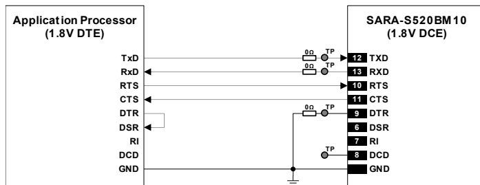
Figure 55: 1 UART interface application circuit with 5-wire link in DTE/DCE serial communication (1.8V DTE)
