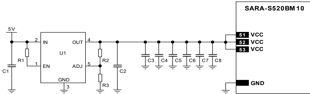
Figure 22: Example of VCC supply circuit for SARA-S520BM10, using an LDO linear regulator
