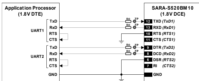
Figure 61: 2 UART interfaces application circuit with 3-wire links in DTE/DCE serial communications (1.8 V DTE)
