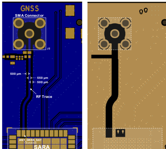
Figure 46: Top layer (L1) and buried layer (L2) layout of the host PCB with the GNSS / Satellite antenna RF trace design
