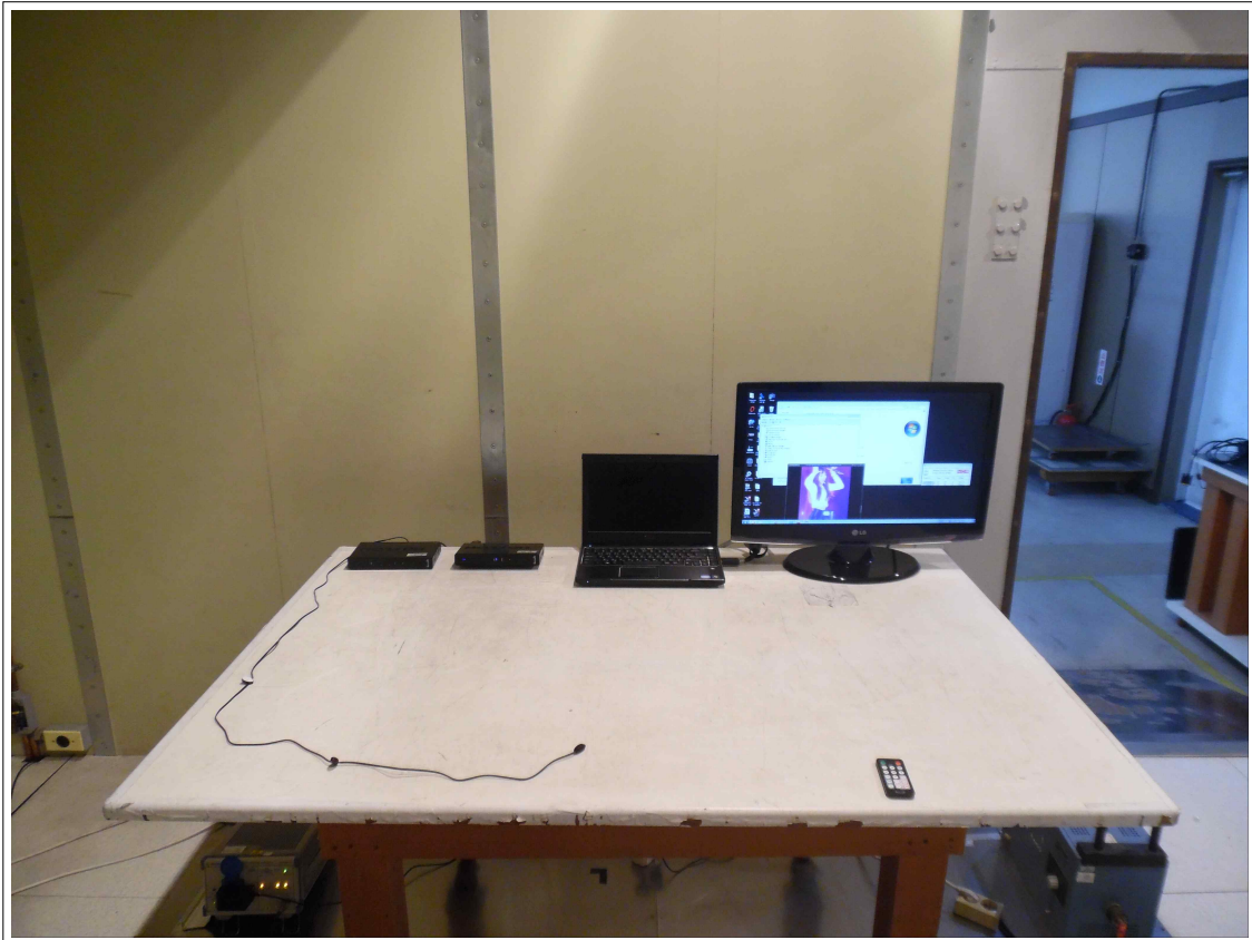
Conducted Disturbance Voltage (Main Port)
