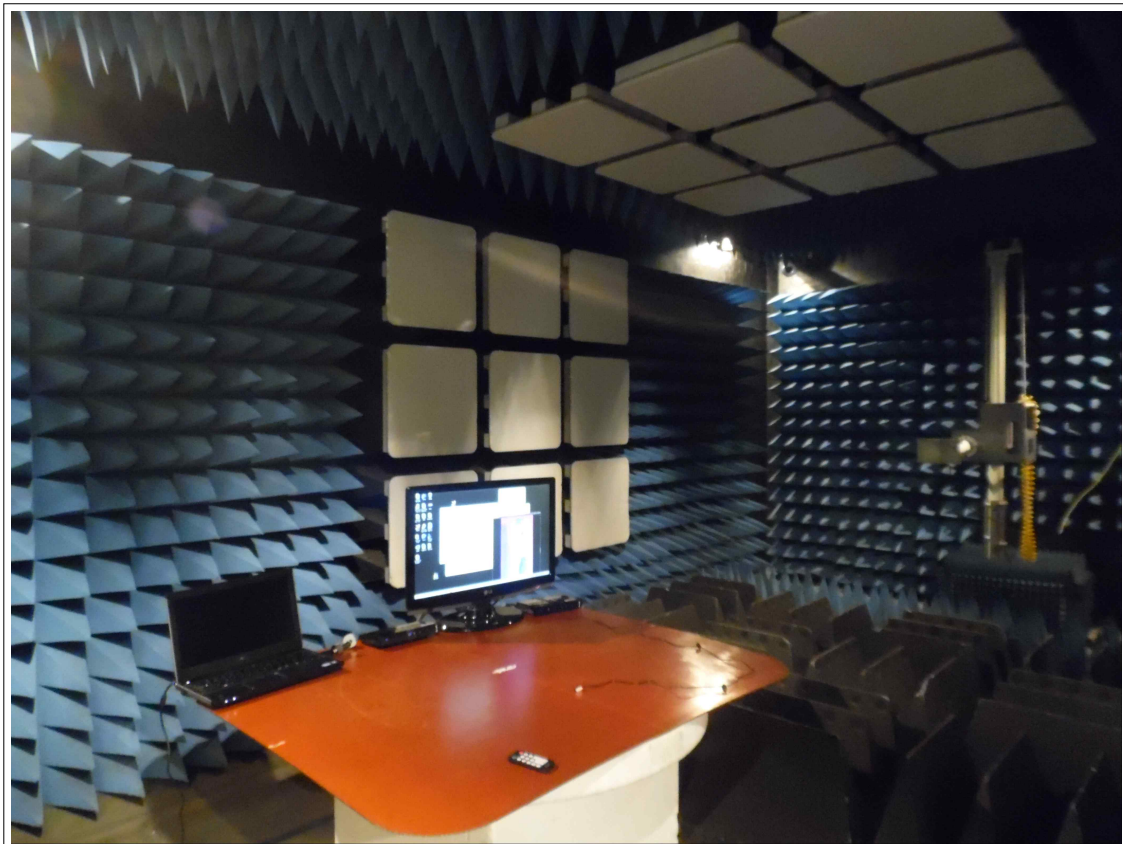
Radiated Electric Field Emissions (Above 1000 MHz)
