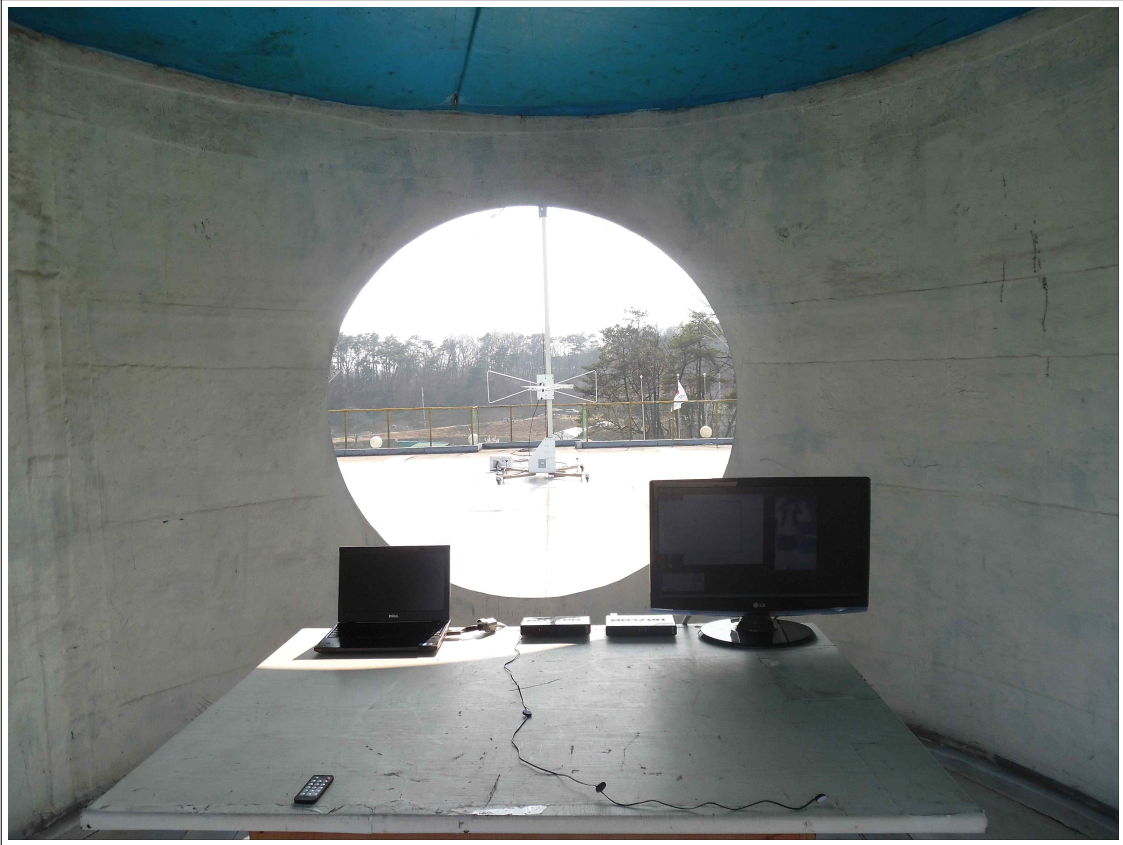
Radiated Electric Field Emissions (Below 1000 MHz)
