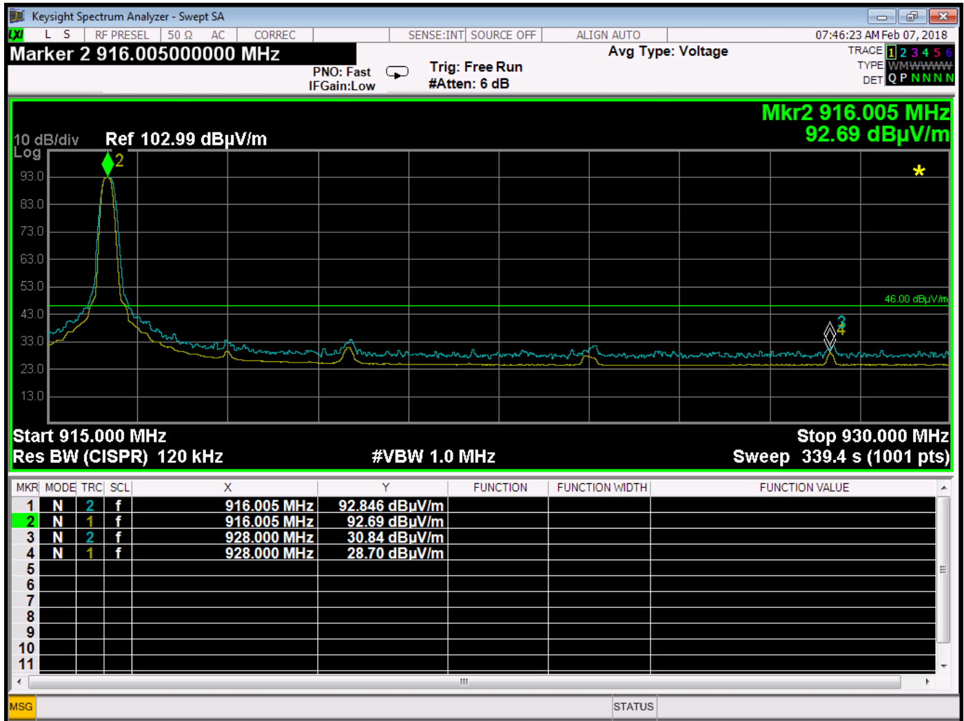
Band Edge - 916 MHz - Horizontal - X-Axis - Worst Case
