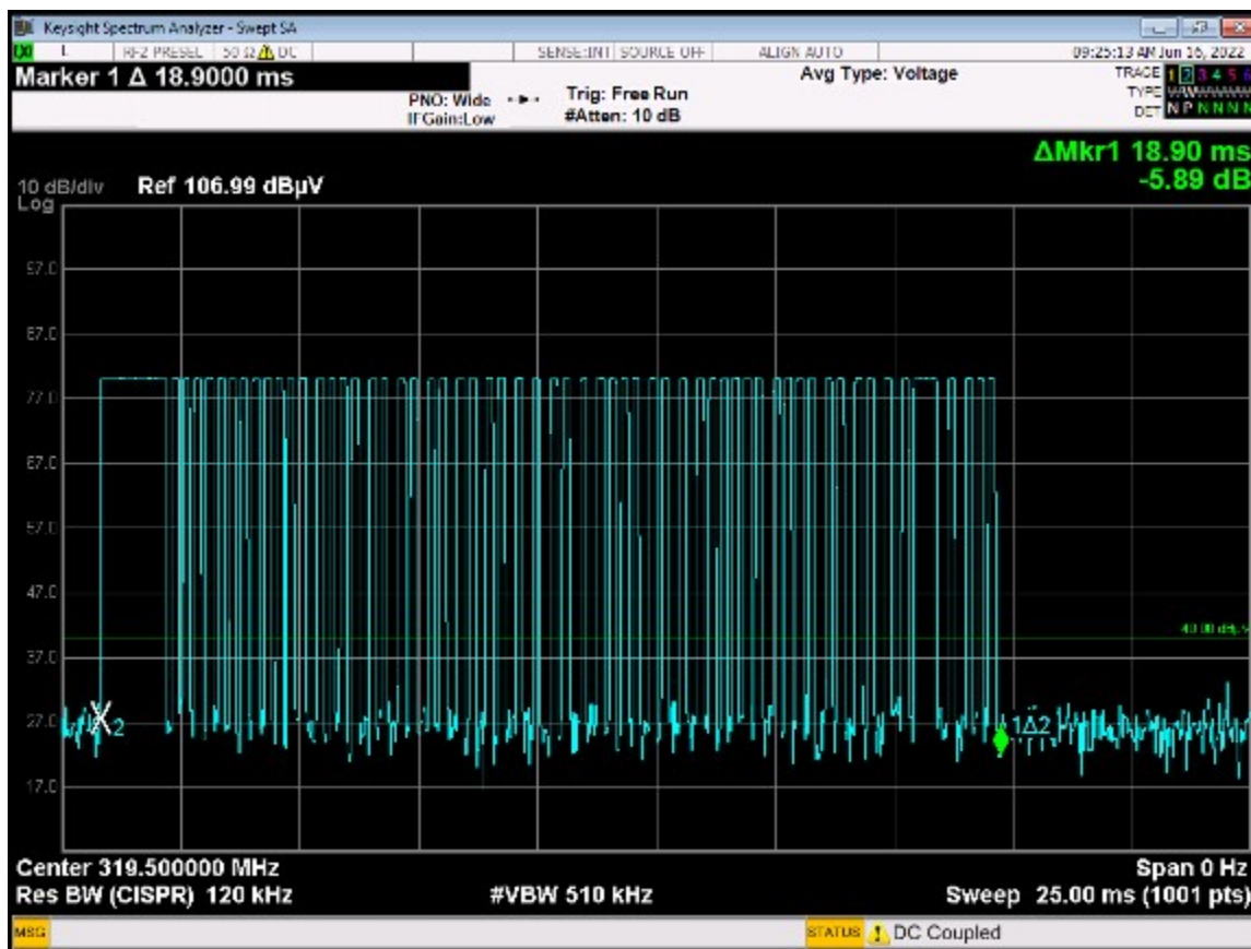
Plot showing the Pulse Train – 58 Small Pulses, 1 Medium Pulse, and 1 Large Pulse
