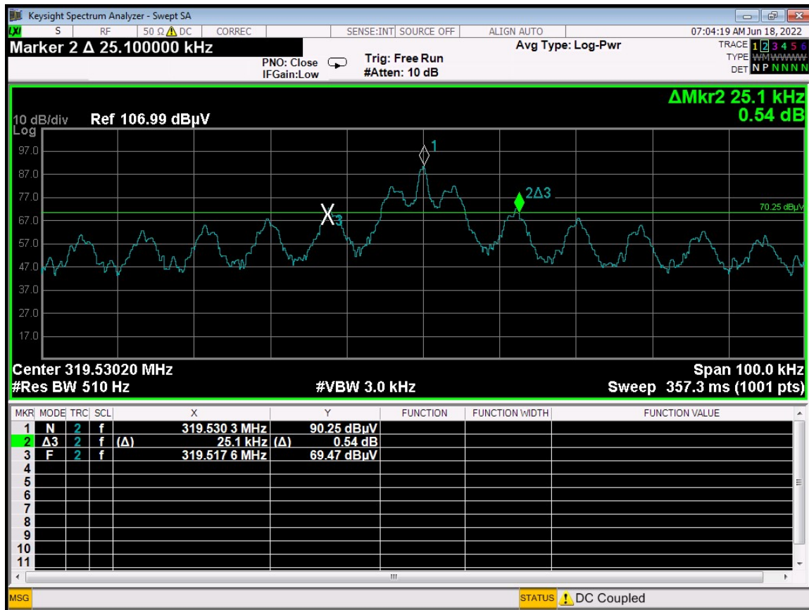
-20 dB Bandwidth Plot - 510 Hz RBW
