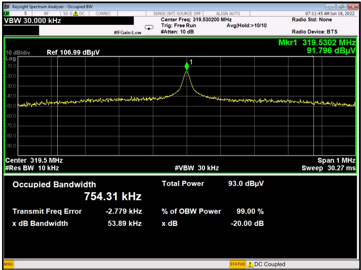
99% Bandwidth Plot
