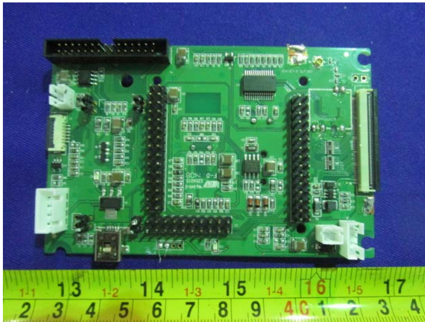
EUT –Ctrl Board Top View
