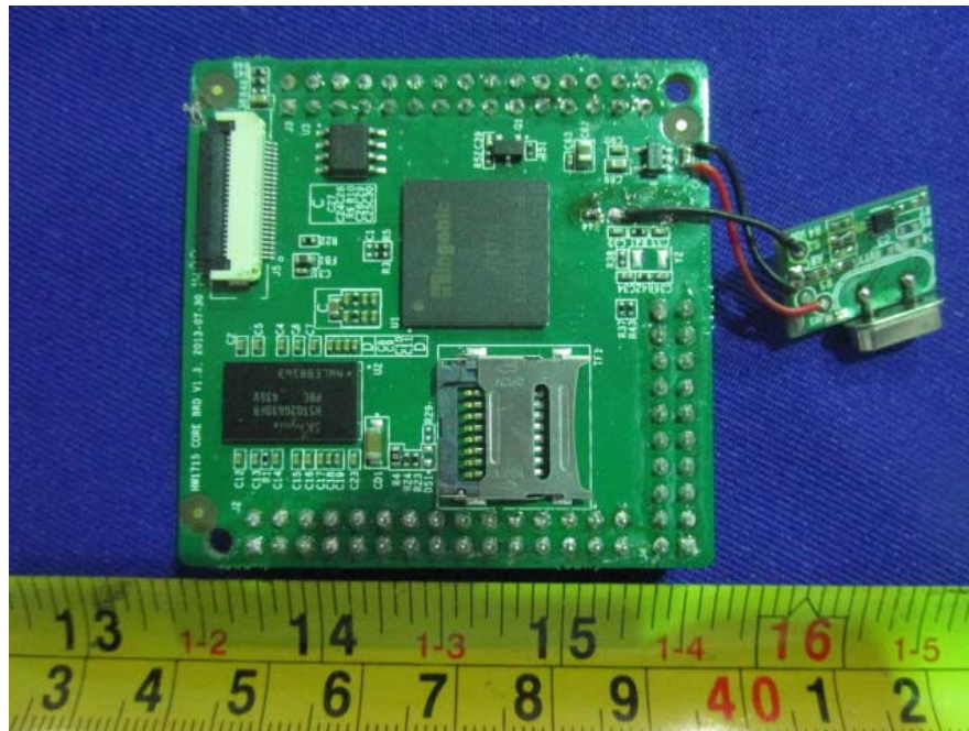
EUT –Core Board Top View
