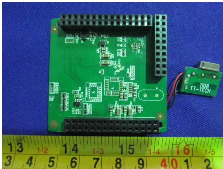
EUT –Core Board Bottom View
