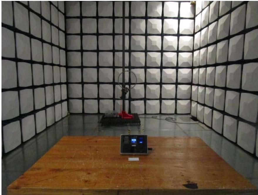
Radiated Emission 9 KHz-30 MHz –View
