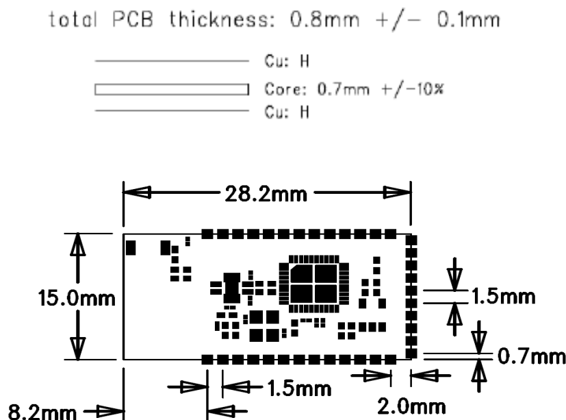
Fig. 22 BTR602 module terminals & shapes of parts
