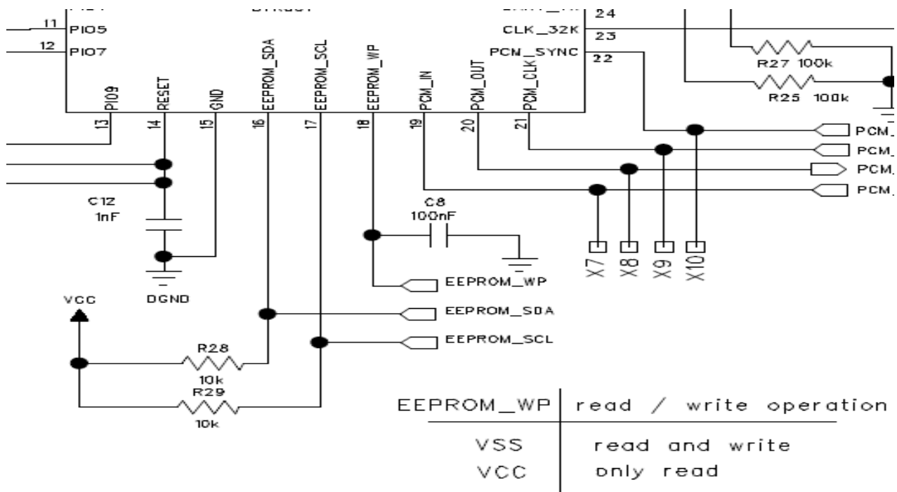
Fig. 8 EEPROM connection
