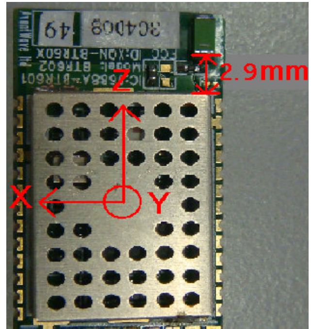
Fig. 15 Laboratory setup environment & BTR602 AUT radiative measurement direction
